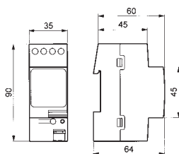
M-Bus Adapter
