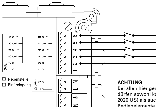
Abb. 7: 24 V ~/- (intern)
