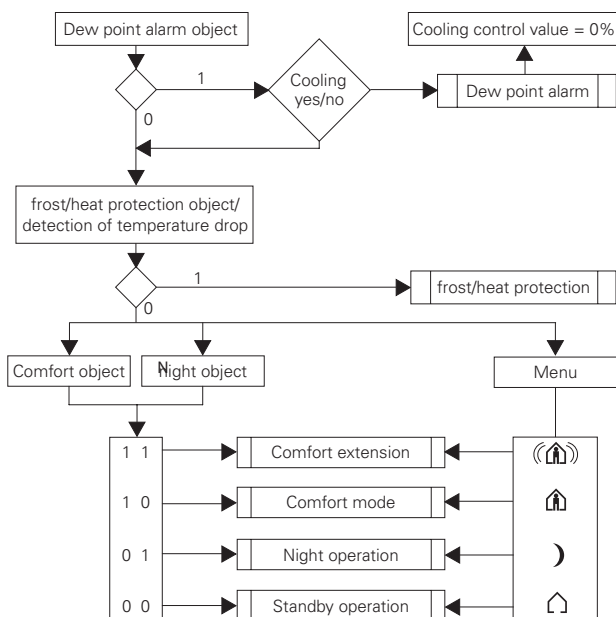
Toggling between operation modes via 1 bit
