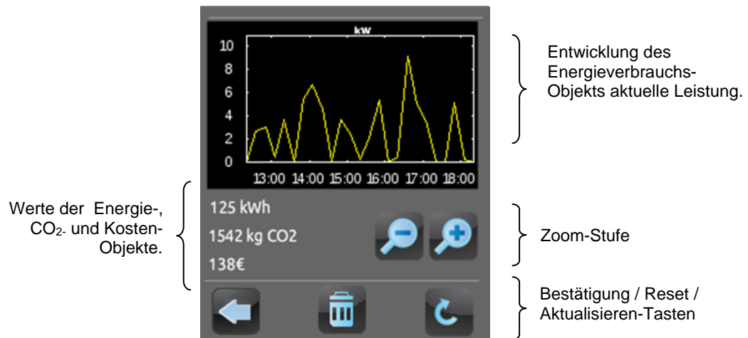
Abb. 68 Energiemonitor (KES). Pop-Up Fenster.
