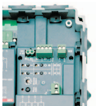
Fig. 2: Manual operation
