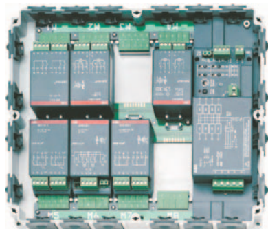
Fig. 1: Open device
