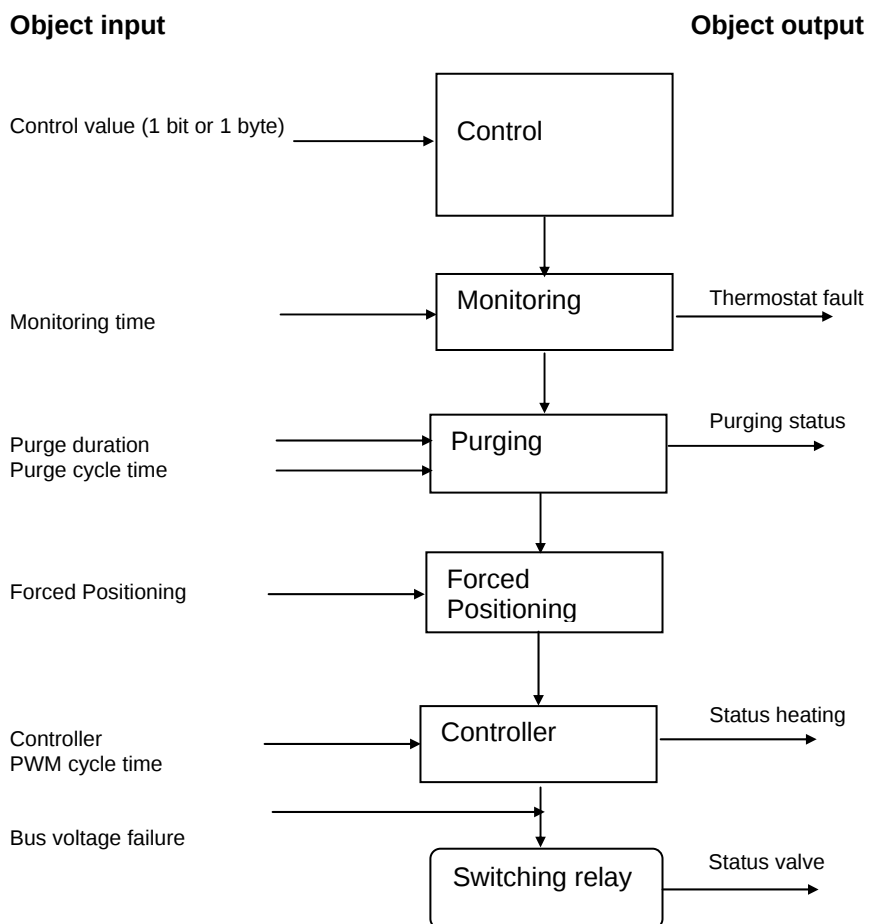
Fig. 39: Function schematic – Control Valve (Heating)
