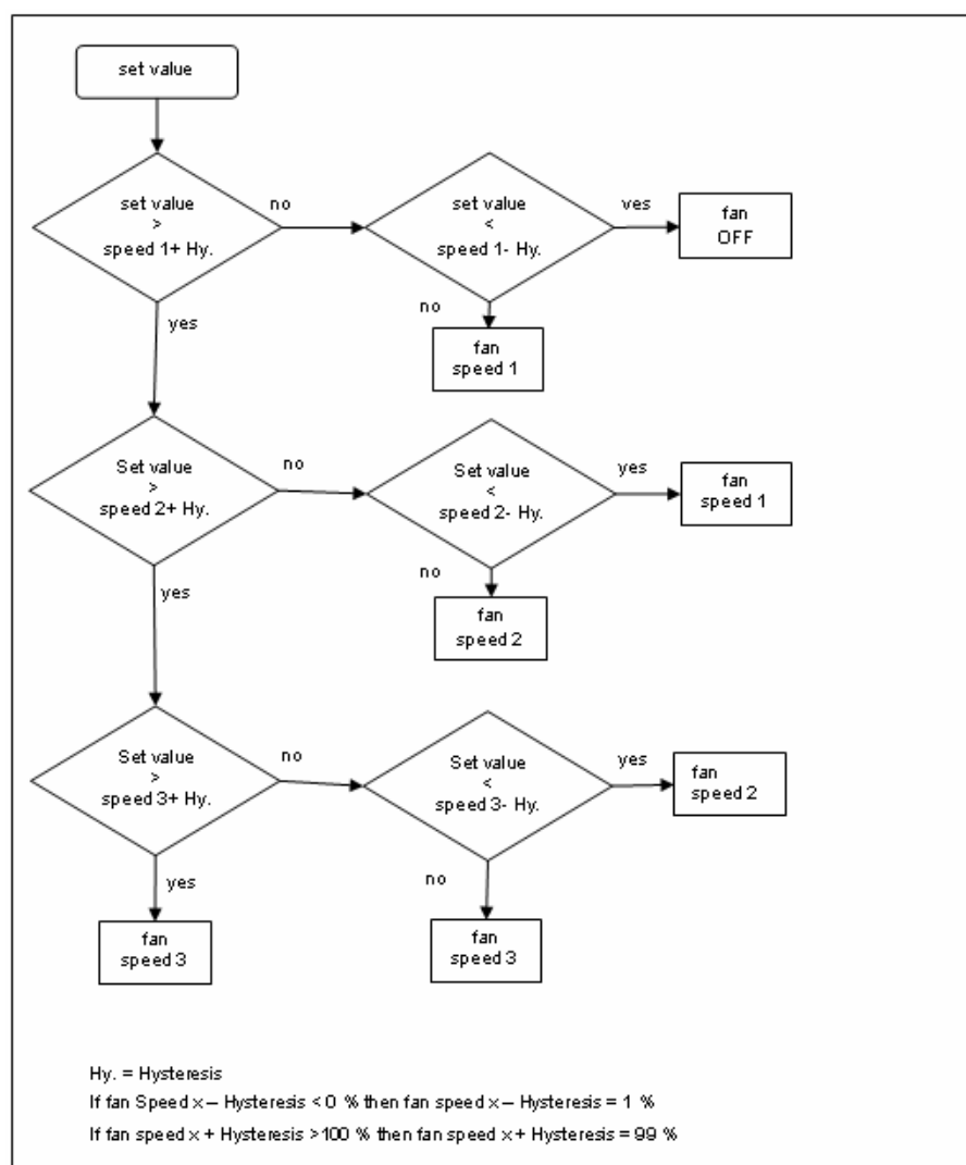
Fig. 36: Logic for changing fan speed
