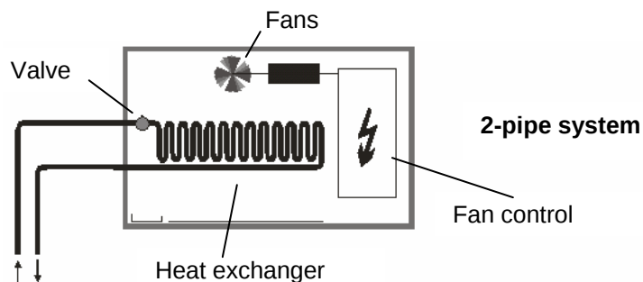
Fig. 27: Design of 2-pipe fan coil unit
