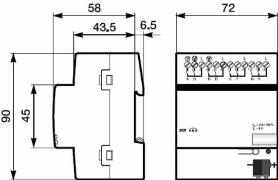
Fig. 7: Dimension drawing LFA/S 2.1
