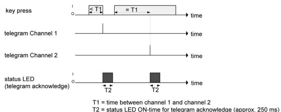
Figure 18: Example of operation concept "Channel 1 or Channel 2"
