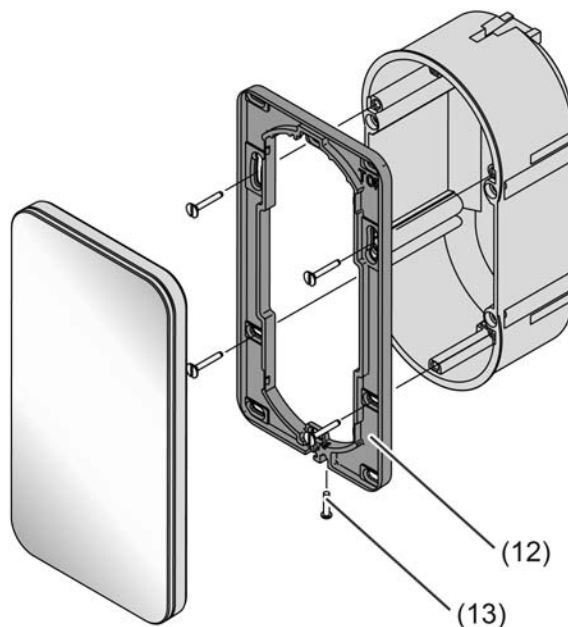
Figure 3: Device mounting of a Comfort touch sensor
