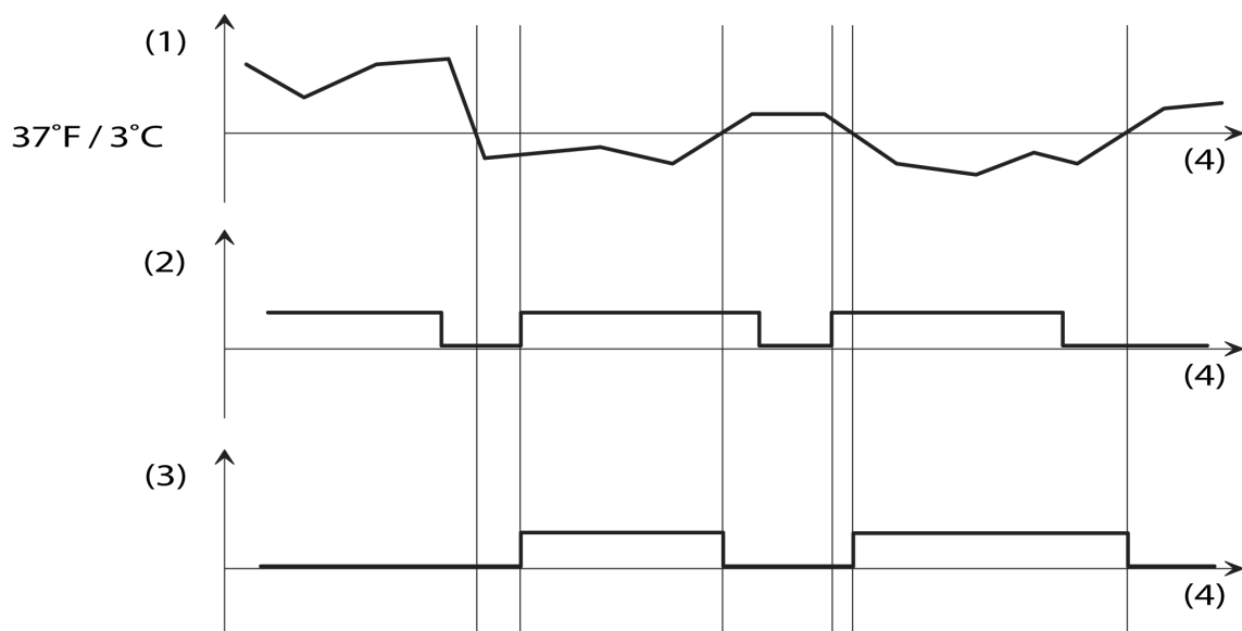
picture 8: Anti-icing protection depending on temperature and precipitation
