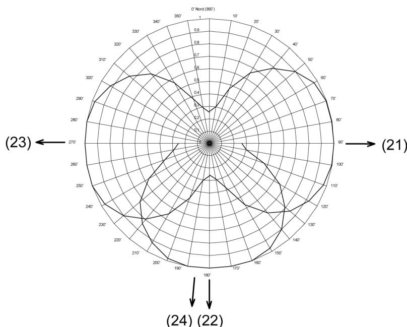
picture 11: Circular chart for brightness detection
