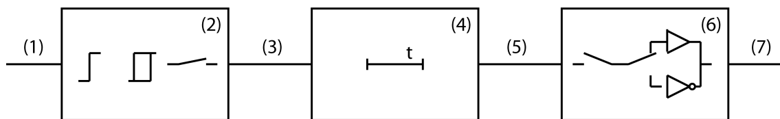
picture 15: Block diagram for switch-on and switch-off delay
