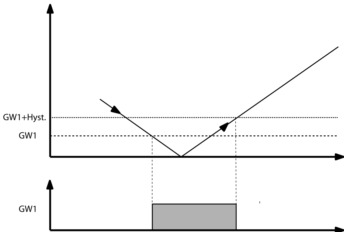
picture 14: Activation of limiting value
