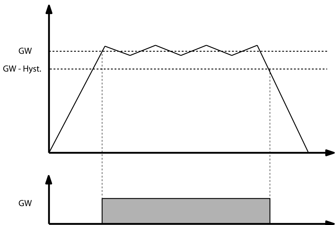
picture 13: Frequency of switching with hysteresis parameterised.
