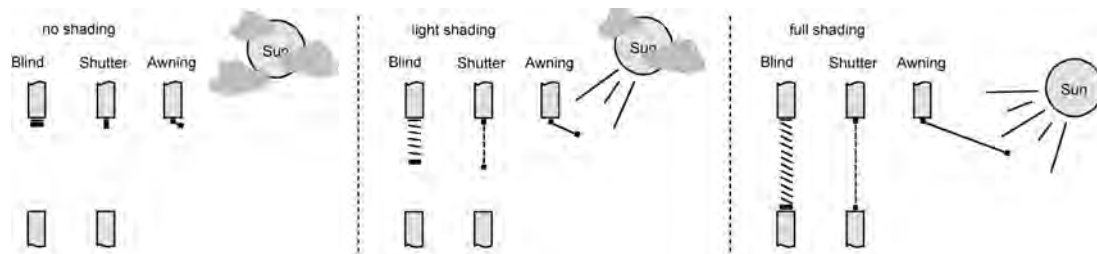
picture 19: Sun protection principles (example)
