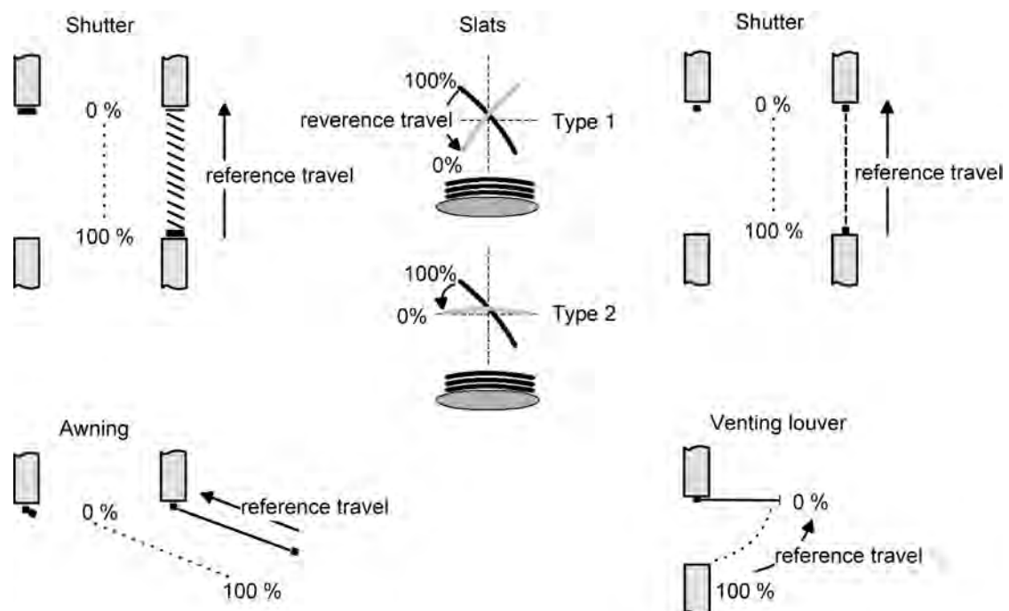
picture 17: Reference movement
