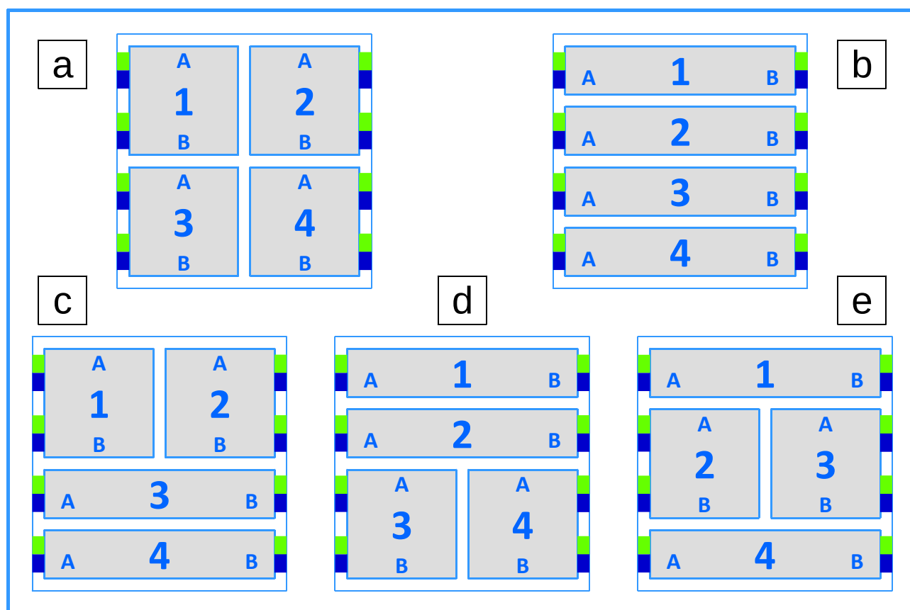
Fig. 7 - Rocker combinations (EK-EA2-TP 4-function)
