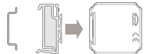
a) Insert the mounting support into the appropriate shaped profile of the interface
