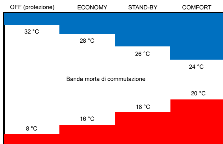
Figure 5 - Deadband and example of consistently distributed setpoint values
