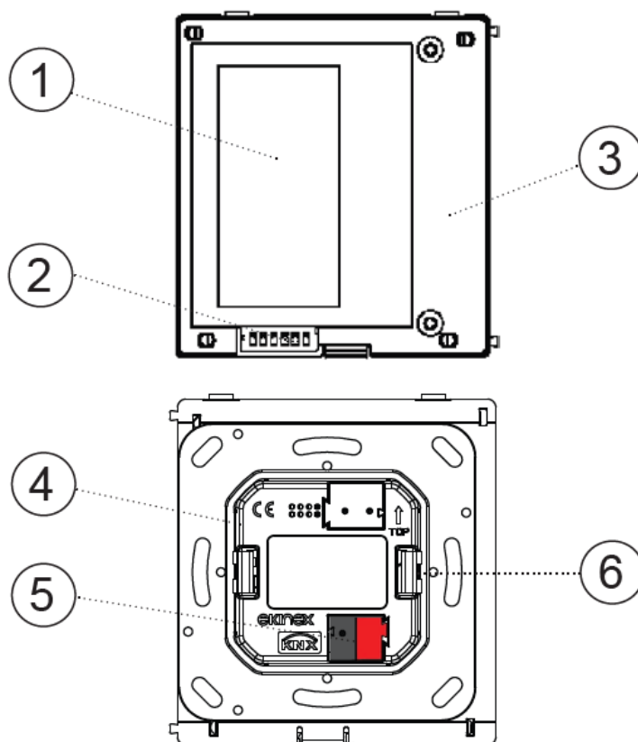
Fig. 2A – Signalling and switching elements
