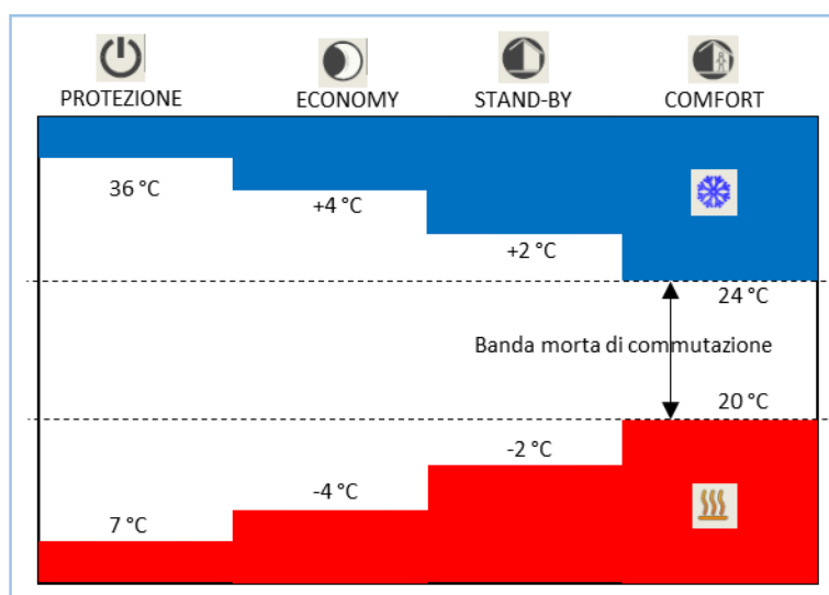
Figure 5 - Deadband and example of consistently distributed setpoint values
