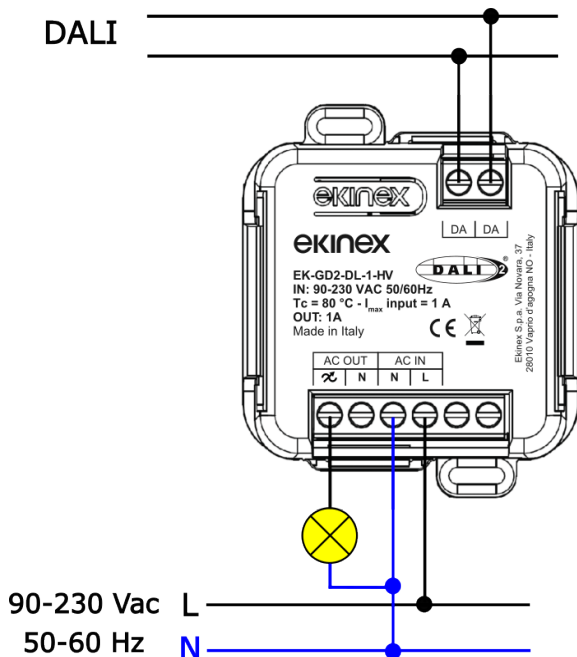
Three-wire connection diagram with common neutral
