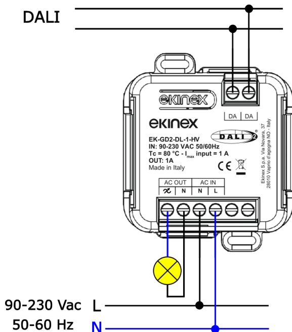
Four-wire connection diagram with phases and neutral reversed
