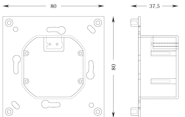
Figure 13: Dimensions of the built-in box – bus coupler
