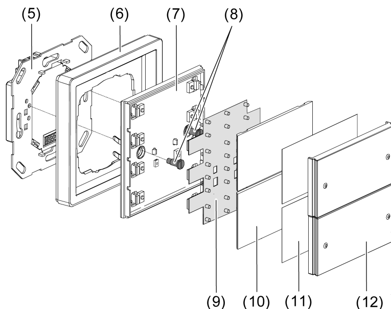
picture 2: Device fitting using the example of a push button sensor 3 basic 2-gang F100
