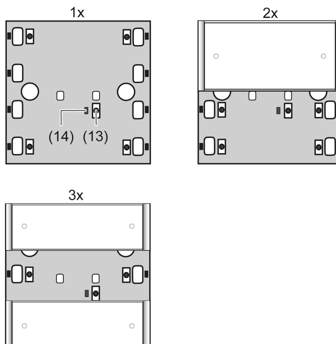
picture 3: Arrangement of the programming button and LED on the front of the device
