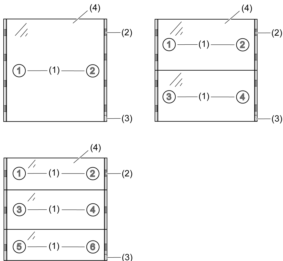
picture 1: Device components of push button sensors 3 basic F100
