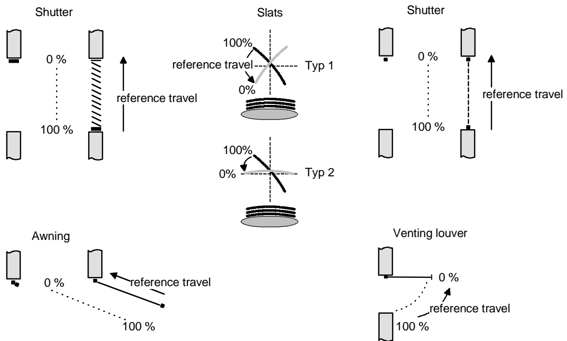
Fig. 29: Reference travel
