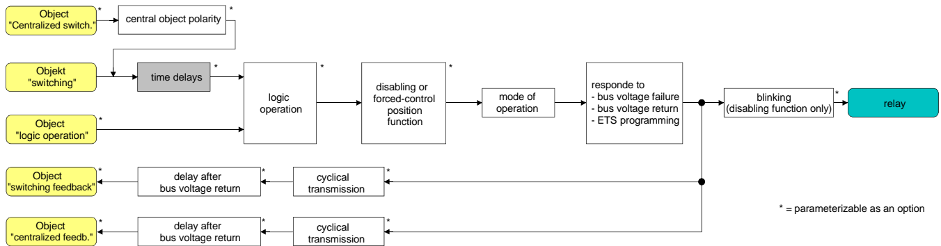
Fig.13: Functional diagram of the time delays
