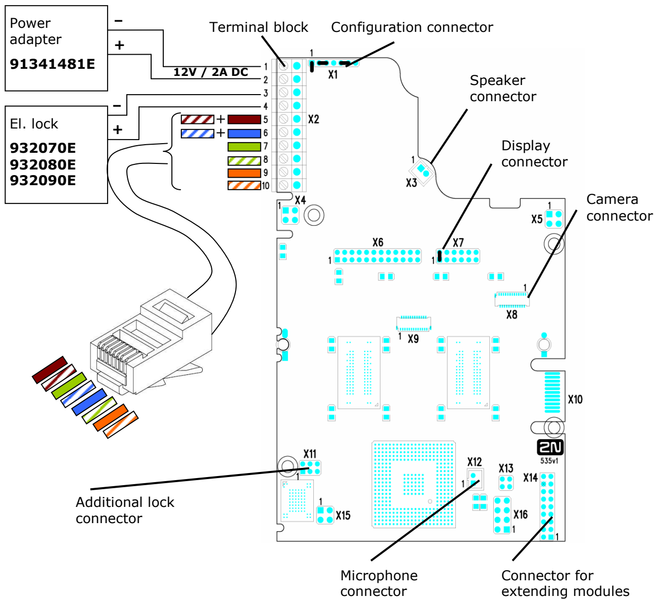
Figure 2.12 Description of 2N® Helios IP Connectors, PCB Versions 535v1, 535v2
