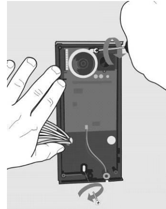
Figure 2.6 Wall Mounting
