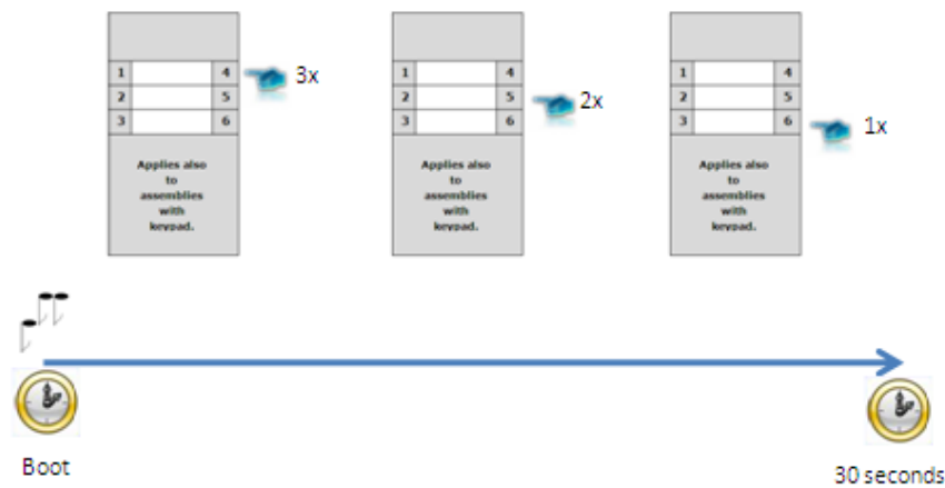
Figure 3.2 Switching to Default Network Parameters – Static IP Address (Part Nos. 9137161E, 9137161CE, 9137161CKE)
