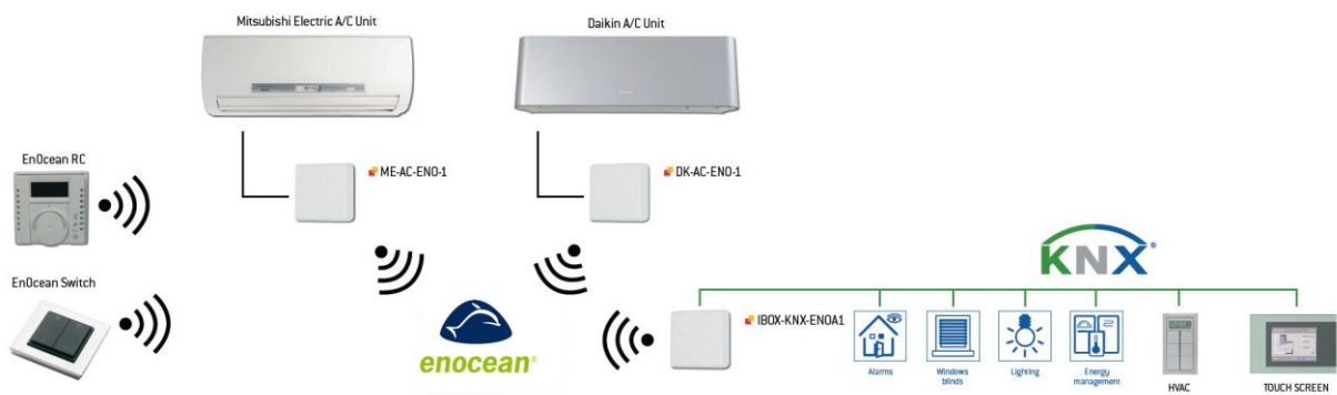
Figure 4.1 IBOX-KNX-ENO-A1 / A1C integration example
