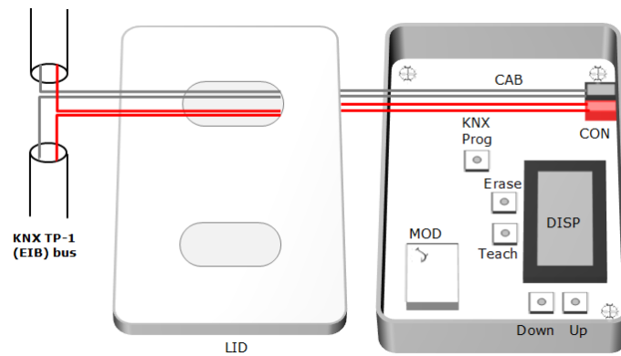
Figure 3.1 IBOX-KNX-ENO-A1 / A1C connection to KNX bus
