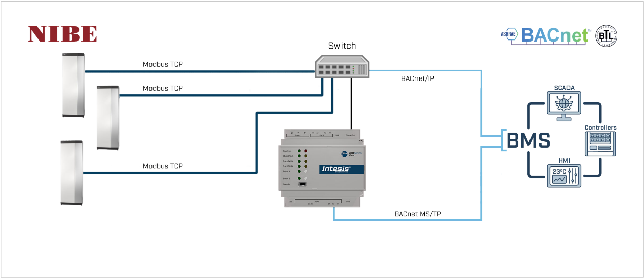
Figure 2. Integration of NIBE heat pumps into BACnet/IP or BACnet MS/TP control systems
