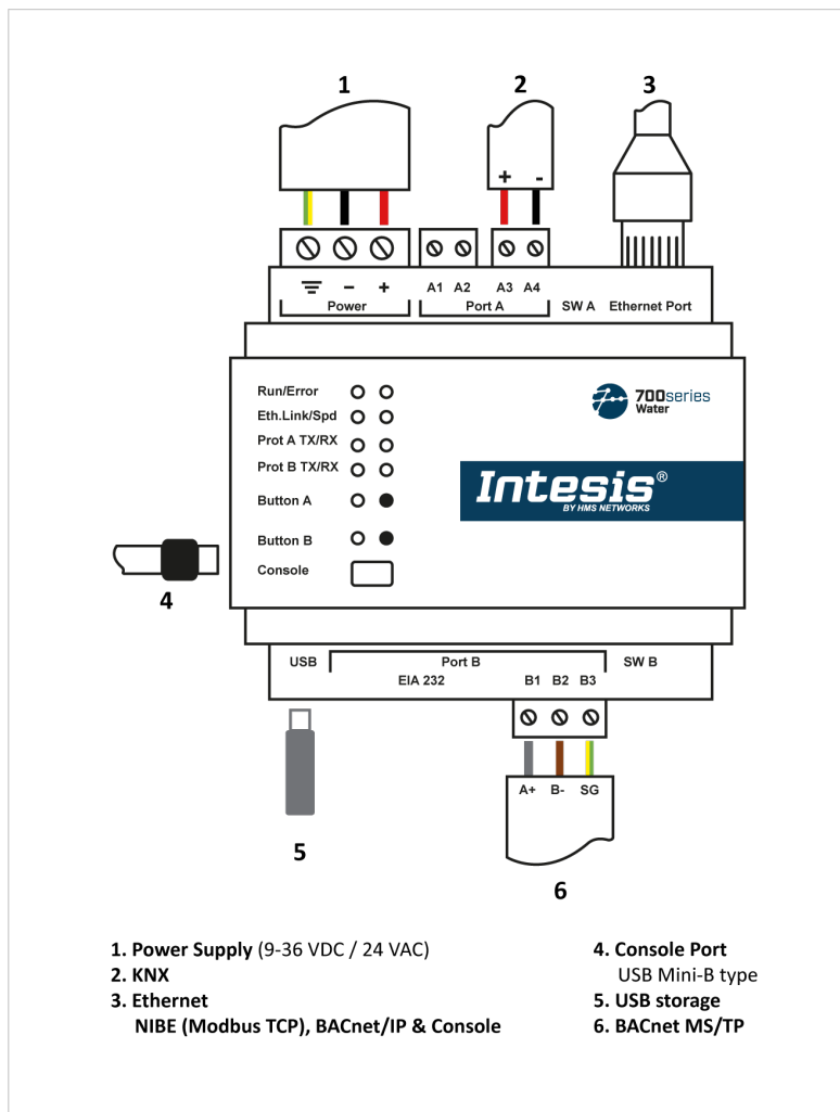
Figure 3. Wiring diagram
