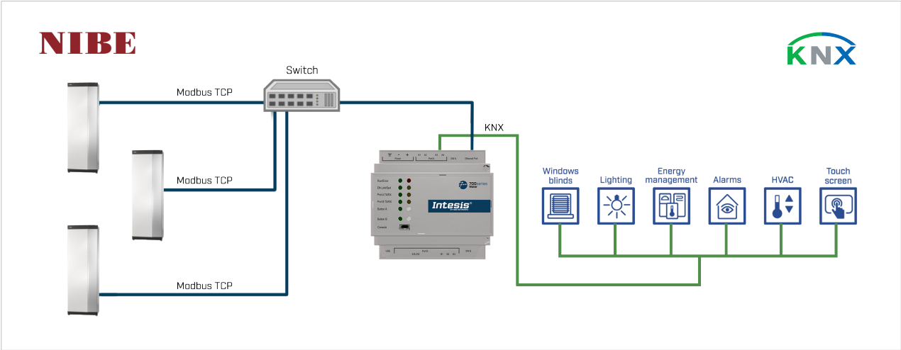
Figure 1. Integration of NIBE heat pumps into KNX TP control systems
