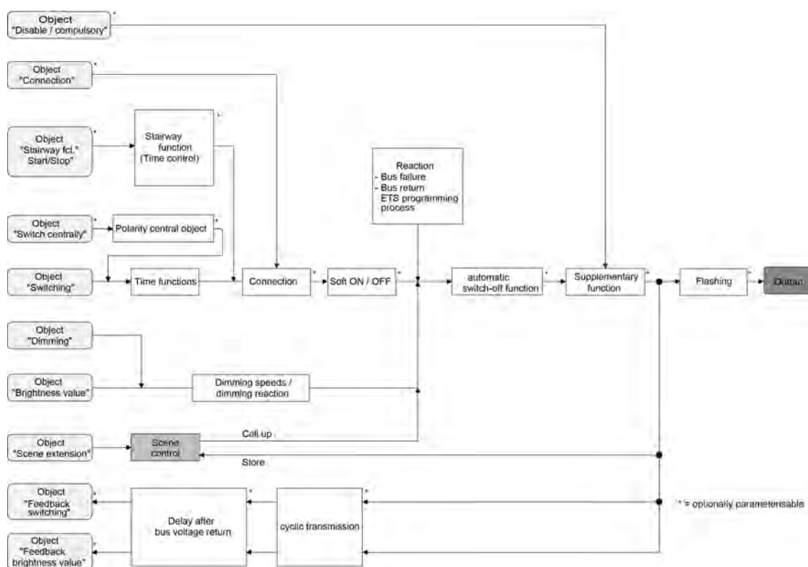
Figure 29: Function diagram of the scene function
