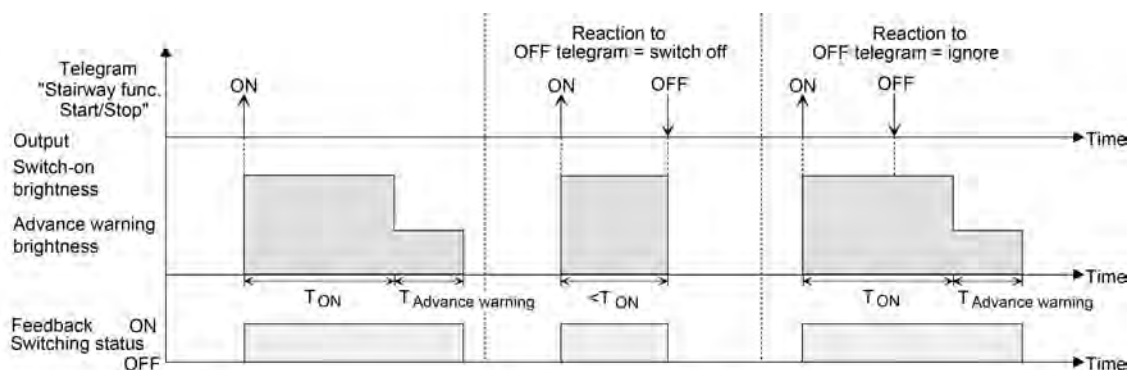
Figure 22: Switch-off behaviour of the staircase function without soft functions
