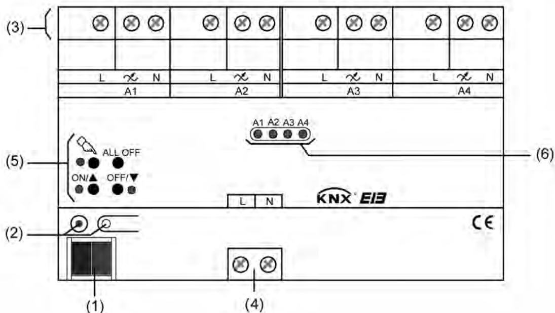
Figure 3: Structure of the 4-gang display variant
