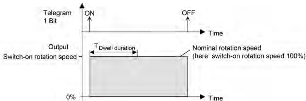
Figure 39: Cutting-in speed and required speed for switching commands
