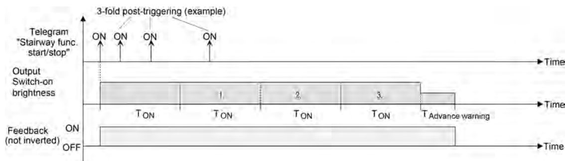
Figure 28: Time extension of the staircase function
