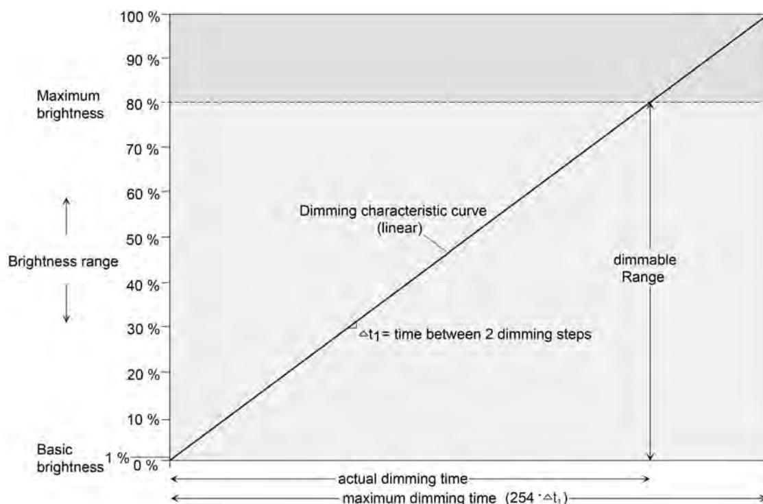
Figure 35: Linear dimming characteristic as an example with basic brightness and maximum brightness
