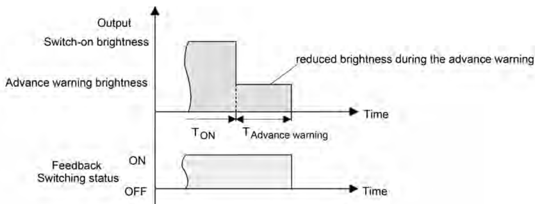
Figure 24: The pre-warning function of the staircase function without soft OFF function
