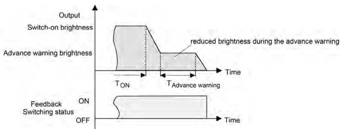
Figure 25: The pre-warning function of the staircase function with soft OFF function (for example with minimum brightness = 0 %)
