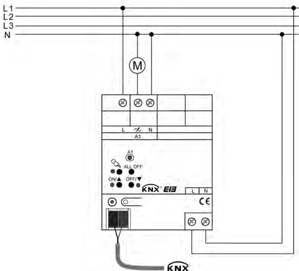
Figure 6: Electrical connection of single-phase electric motors
