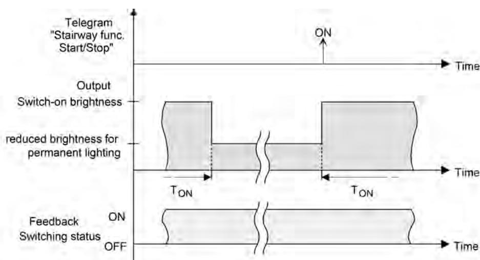
Figure 26: The continuous lighting of the staircase function without soft functions
