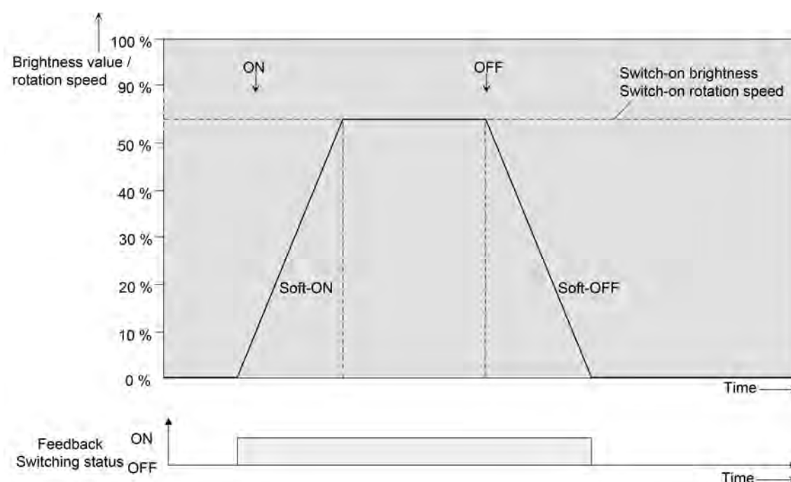
Figure 15: Dimming behaviour of the soft ON/OFF functions (as an example)
