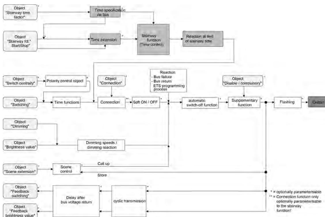
Figure 19: Function diagram of the staircase function
