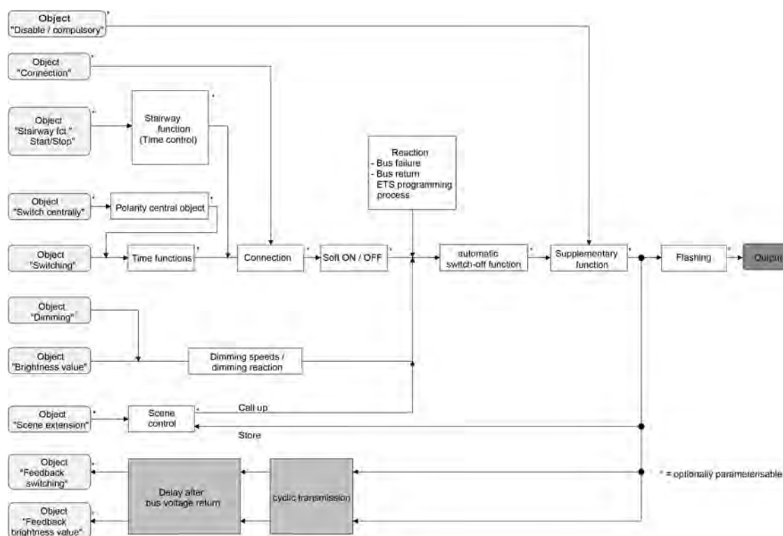
Figure 13: Functional feedback diagram of the feedbacks
