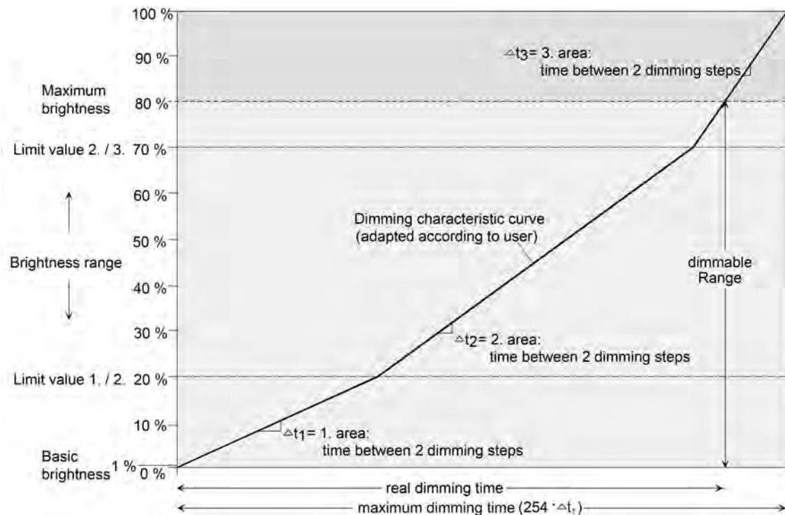
Figure 37: User-defined dimming characteristic as an example with basic brightness and maximum brightness
