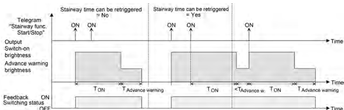
Figure 20: Switch-on behaviour of the staircase function without soft functions
