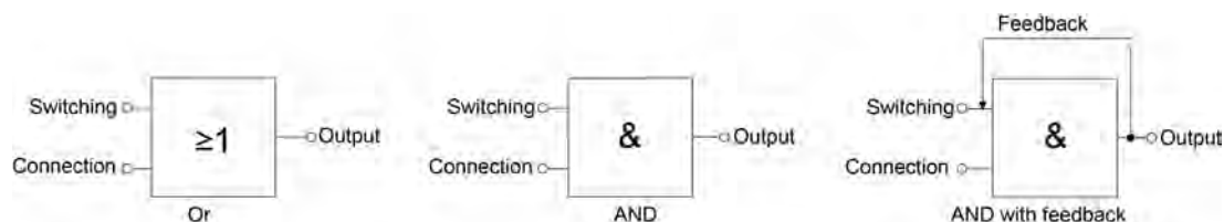
Figure 34: Logic operation types of the logic operation function
