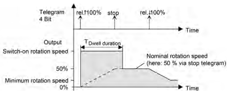
Figure 41: Cutting-in speed and required speed for relative dimming commands
