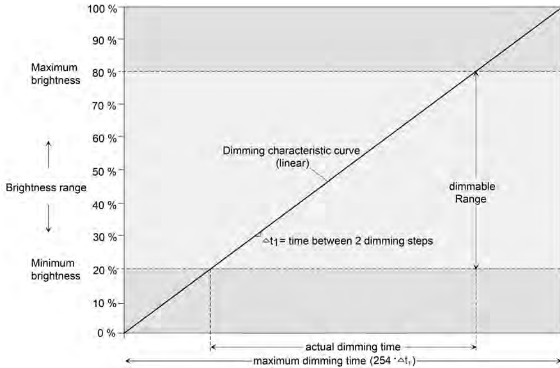
Figure 36: Linear characteristic dimming curve as an example with minimum brightness > 0 % and maximum brightness
