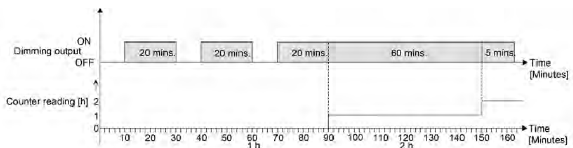
Figure 30: Function of the operating hours counter (using the example of an up-counter)
