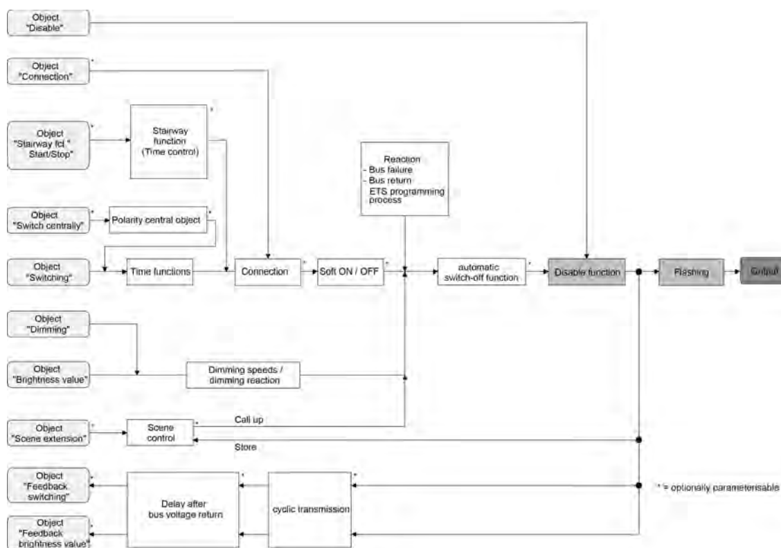
Figure 31: Function diagram of the disabling function
