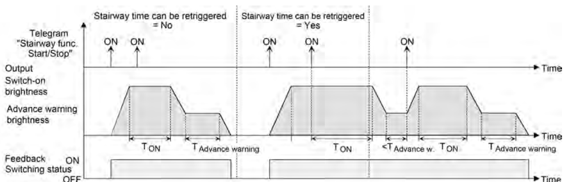
Figure 21: Switch-on behaviour of the staircase function with soft functions (for example with minimum brightness = 0 %)
