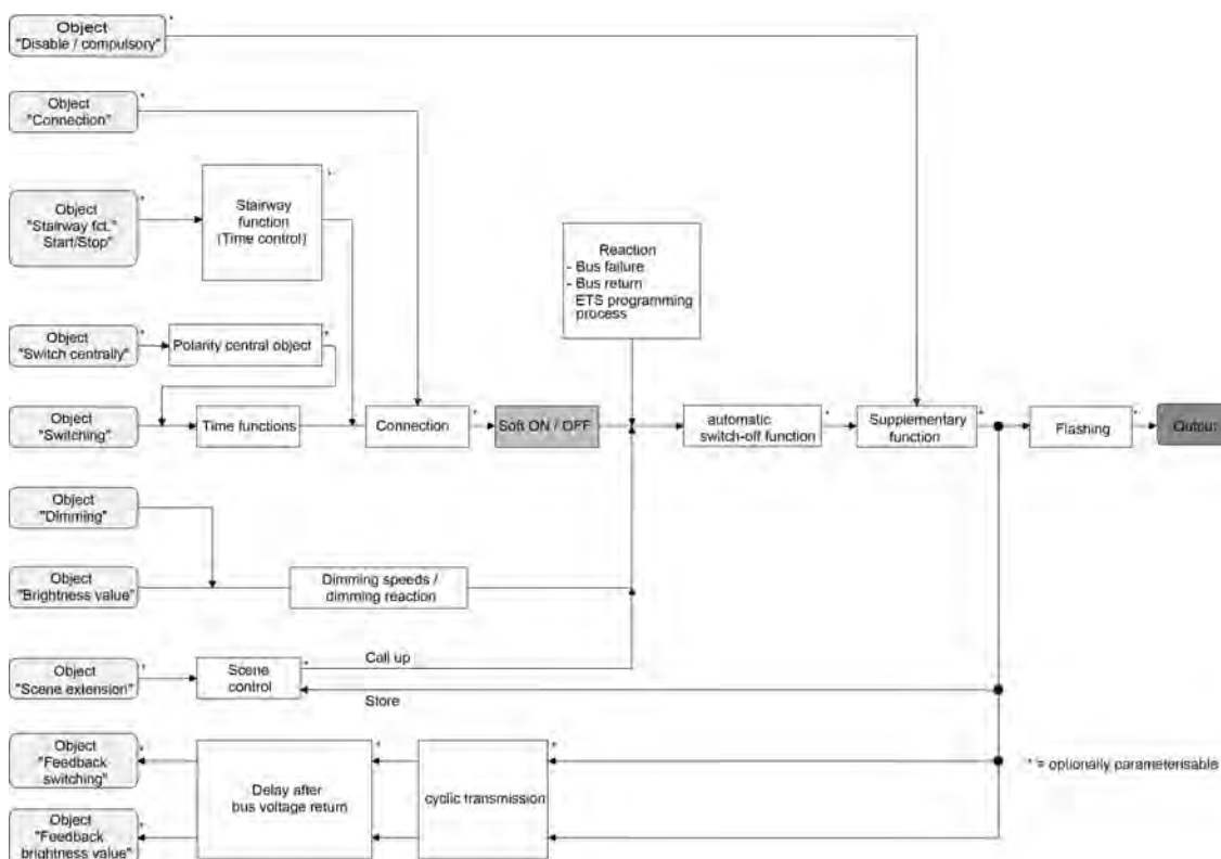
Figure 16: The function diagram of the soft functions
