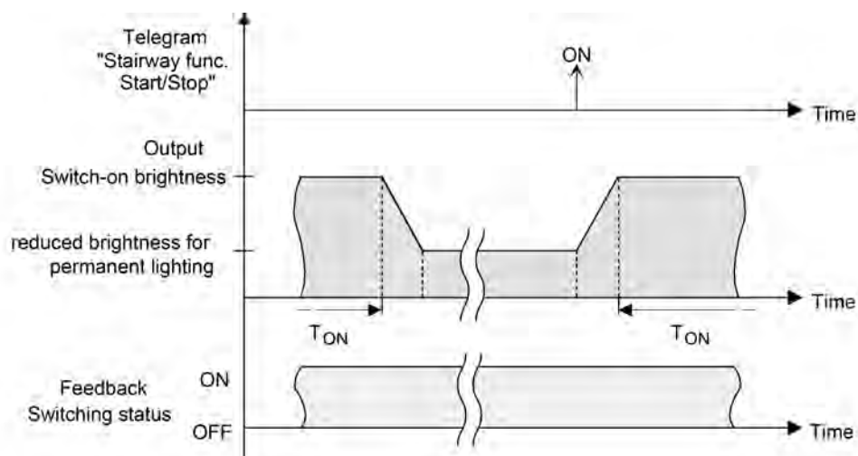
Figure 27: The continuous lighting of the staircase function with soft OFF functions
