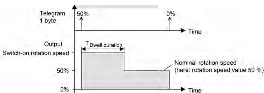
Figure 40: Cutting-in speed and required speed for value commands
