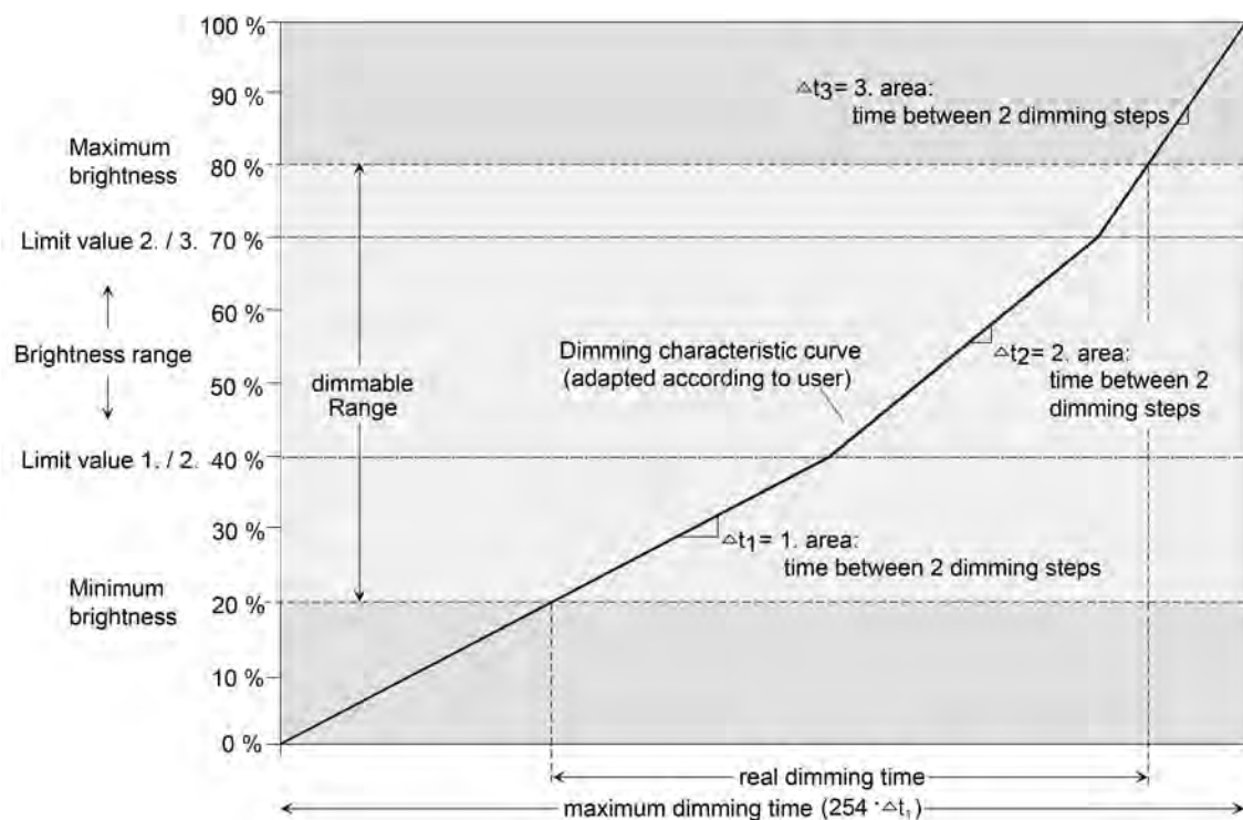
Figure 38: User-defined dimming characteristic as an example with minimum brightness and maximum brightness
