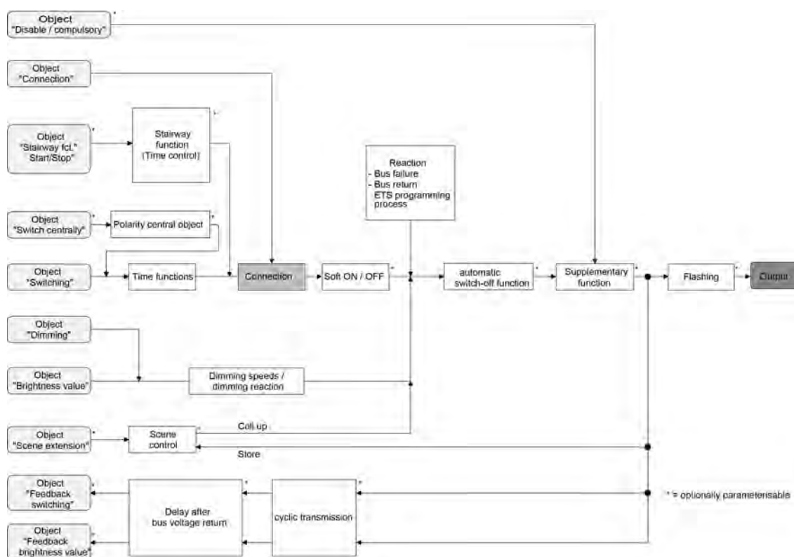
Figure 33: Function diagram of the logic operation function
