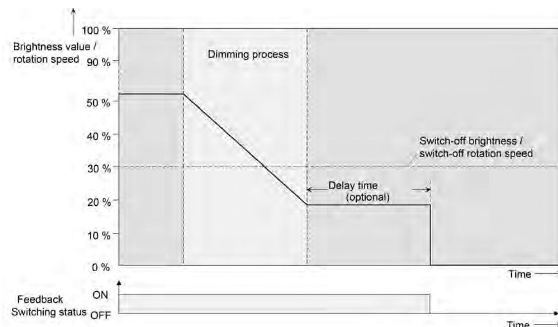
Figure 17: Dimming and switching behaviour of the automatic switch-off function
