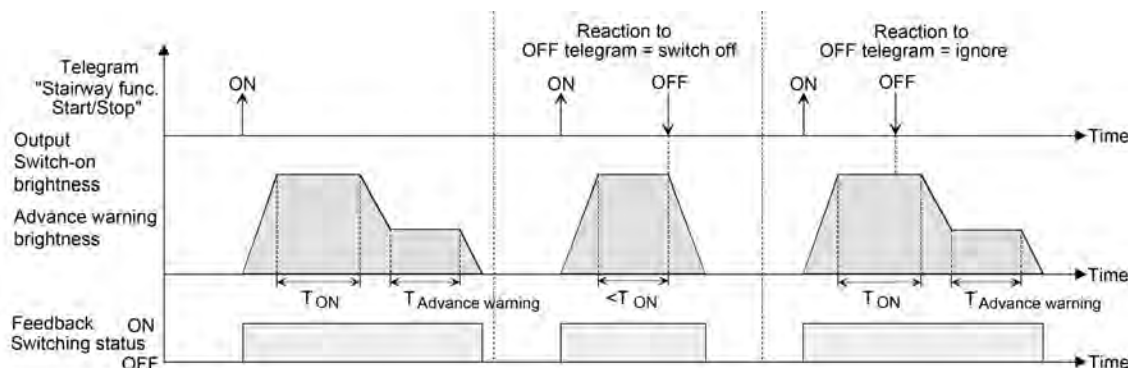
Figure 23: Switch-off behaviour of the staircase function with soft functions (for example with minimum brightness = 0 %)
