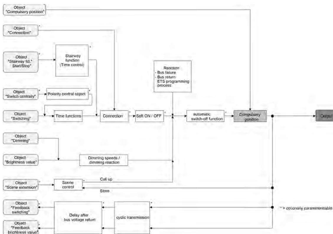
Figure 32: Function diagram of the forced position function
