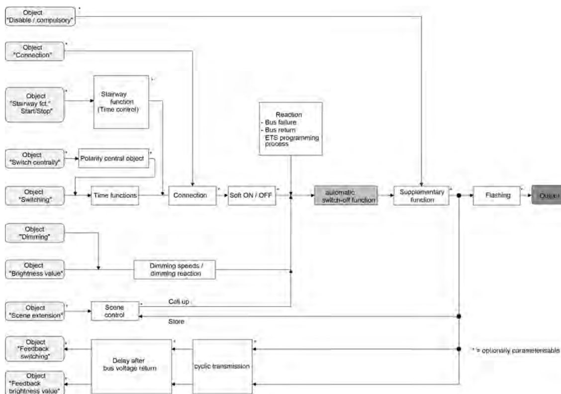
Figure 18: Function diagram of the automatic switch-off function
