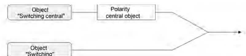
Figure 10: Function diagram "Central switching"
