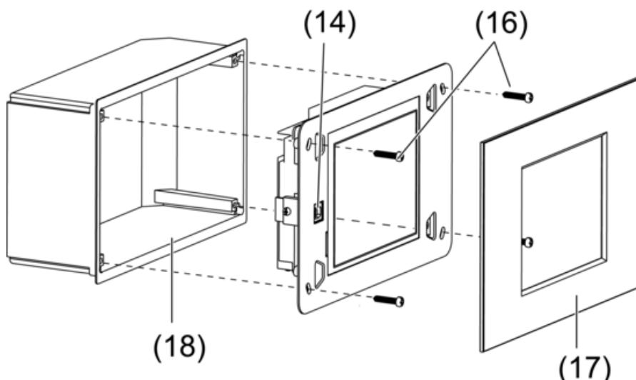
picture 5: Installation in panel-mounted housing.
