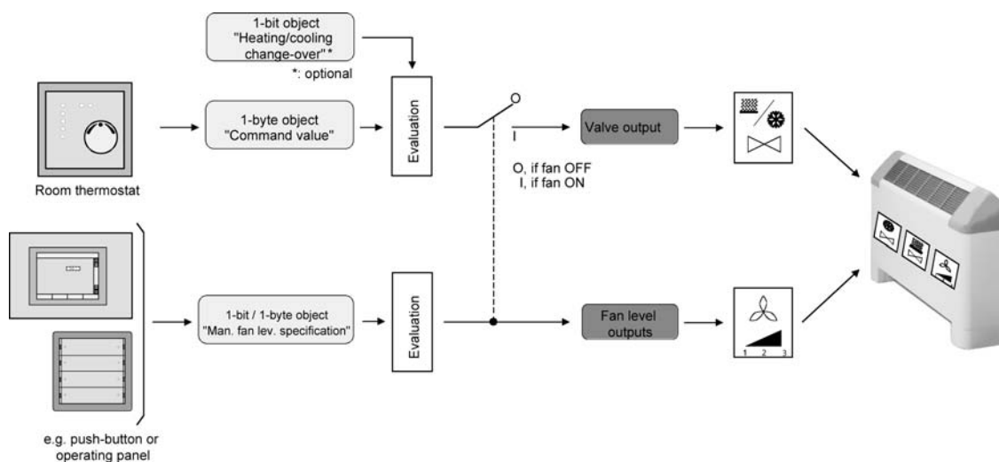
picture 29: Schematic diagram for manual fan control independent of active heating / cooling (simplified depiction)
