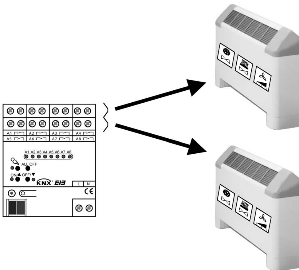
picture 11: 2-channel operation
