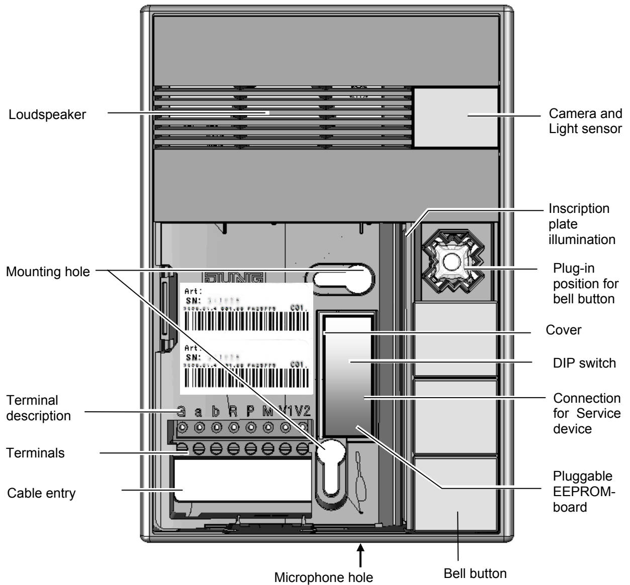
Illustration: TK AS AL 114 A, without inscription plate
