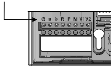
Terminal connections
