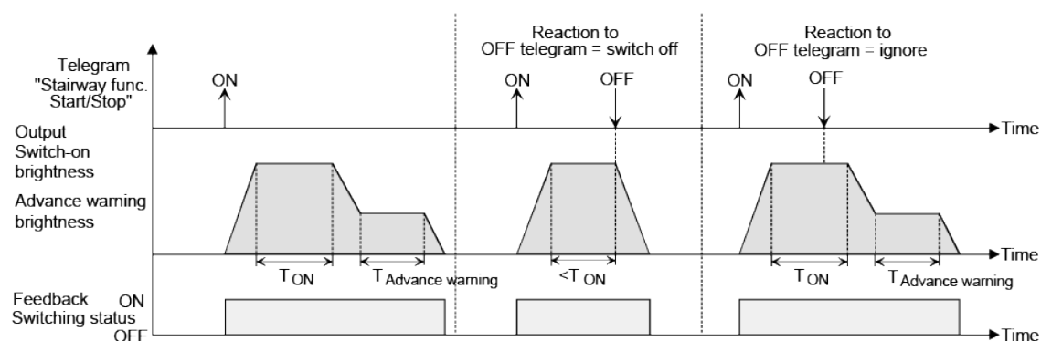
Figure 53: Switch-off behaviour of the staircase function with soft functions (as an example with minimum brightness = 0 %)
