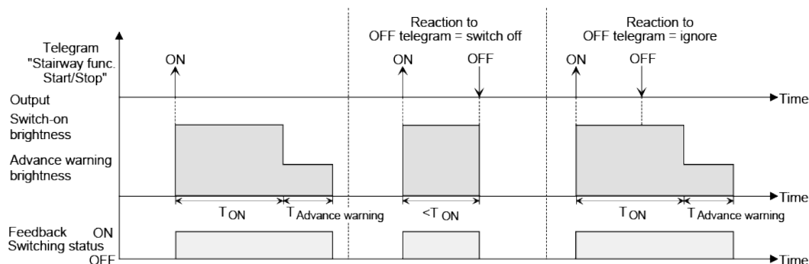
Figure 52: Switch-off behaviour of the staircase function without soft functions
