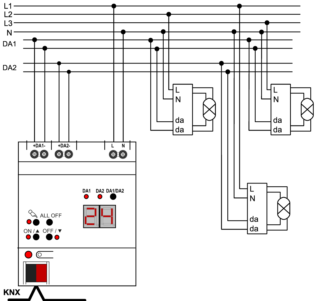
Figure 2: DALI gateway connection example, 2fold
