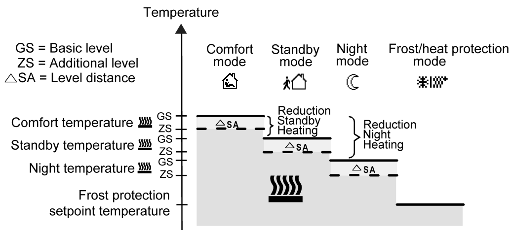
Figure 58: Setpoint temperatures in the operating mode "Basic and additional heating"
