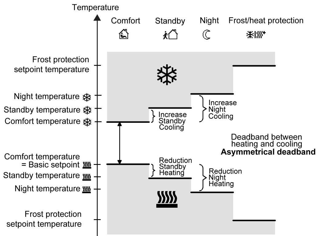
Figure 62: Setpoint temperatures in the operating mode "Heating and cooling" with asymmetrical deadband
