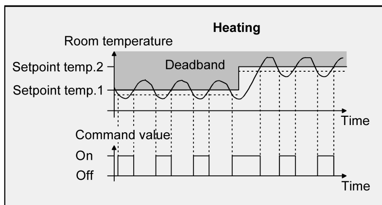
Figure 52: 2-point feedback control for mixed "Heating and cooling" mode with active heating mode
