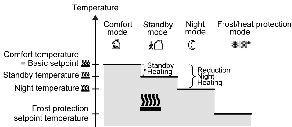
Figure 57: Setpoint temperatures in the operating mode "Heating"
