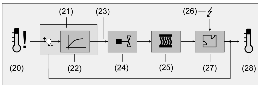
Figure 47: Controlled system of single-room temperature control
