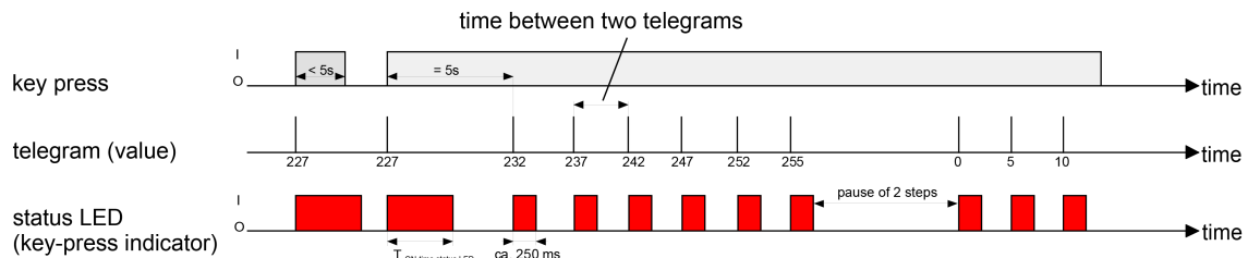
Figure 40: Example of value adjustment with value range overflow
