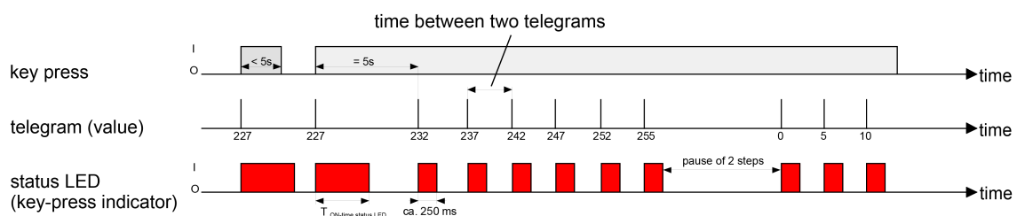
Figure 44: Example of value adjustment with value range overflow
