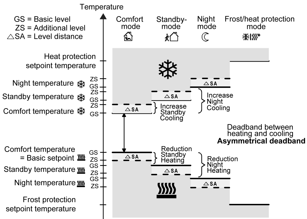
Figure 64: Setpoint temperatures in the operating mode "Basic and additional heating and cooling" with asymmetrical deadband
