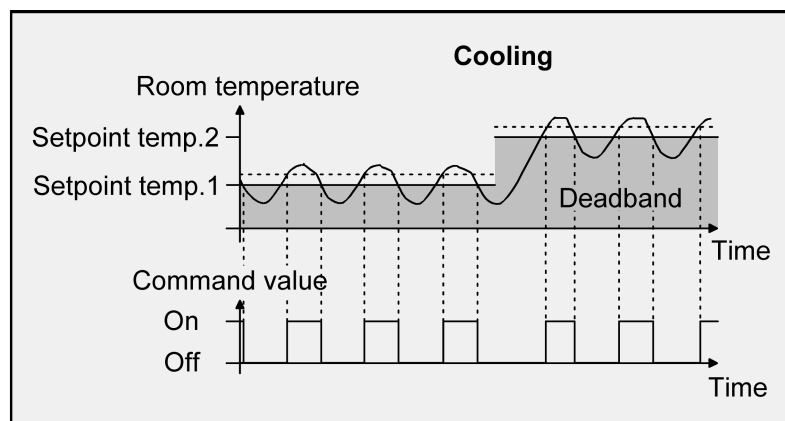
Figure 53: 2-point feedback control for mixed "Heating and cooling" mode with active cooling operation
