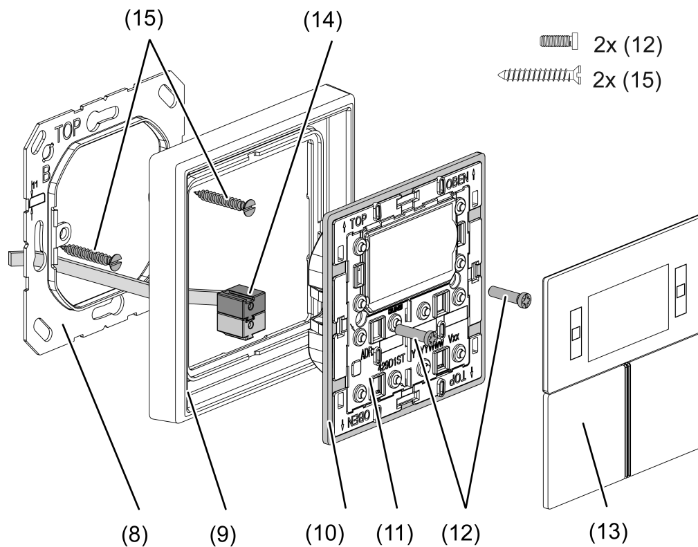
Figure 3: Mounting the controller module
