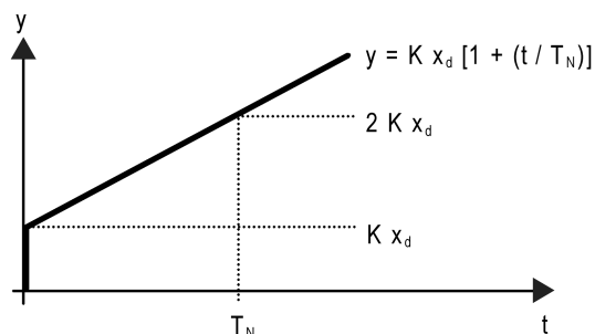
Figure 49: Function of the command value of a PI control
