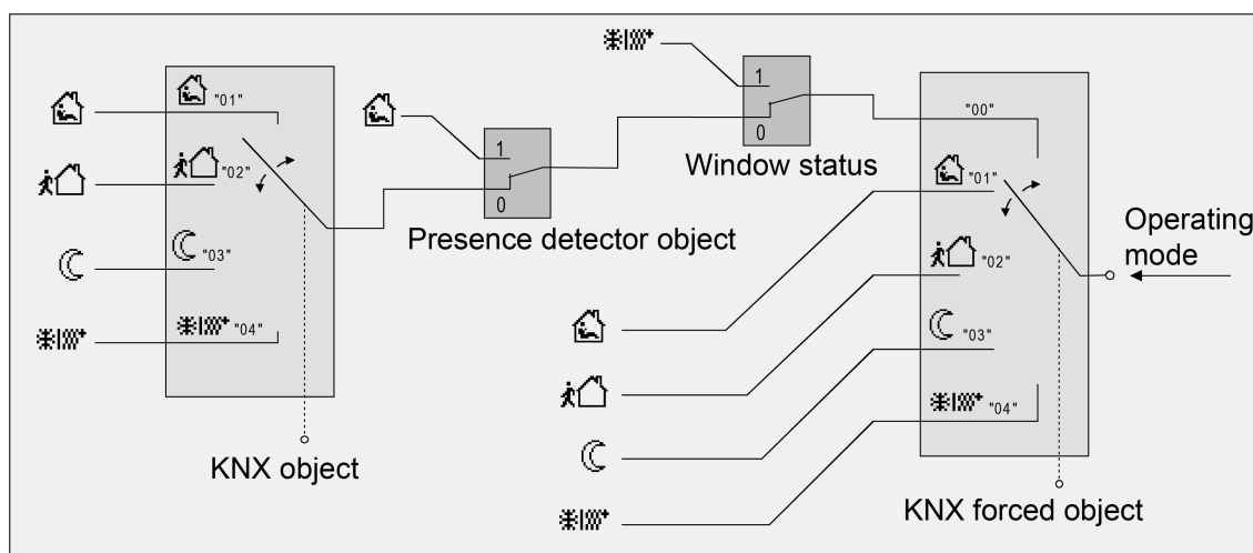
Figure 56: Operating mode switchover through KNX object with presence detector
