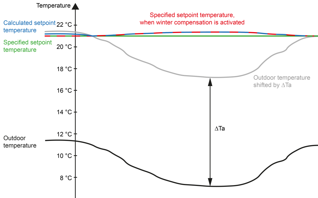
Figure 65: Example for winter compensation
