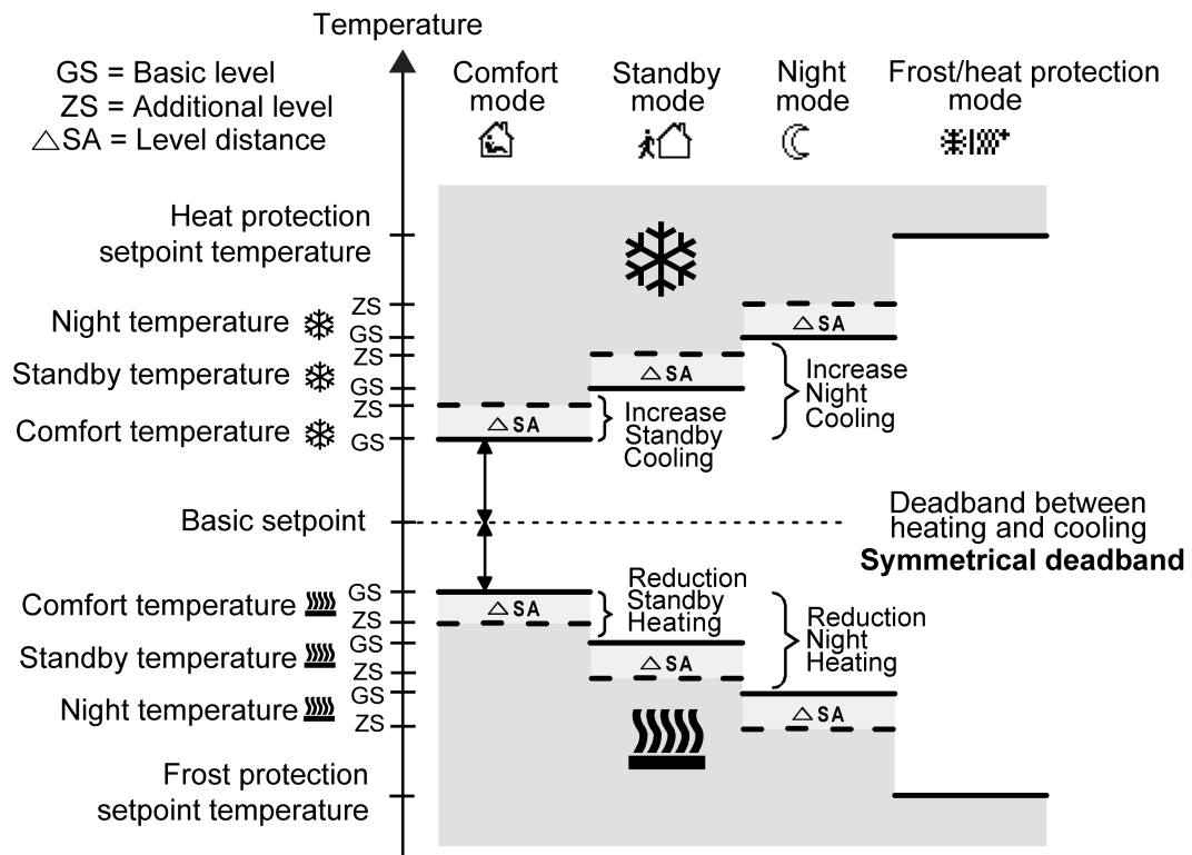
Figure 63: Setpoint temperatures in the operating mode "Basic and additional heating and cooling" with symmetrical deadband
