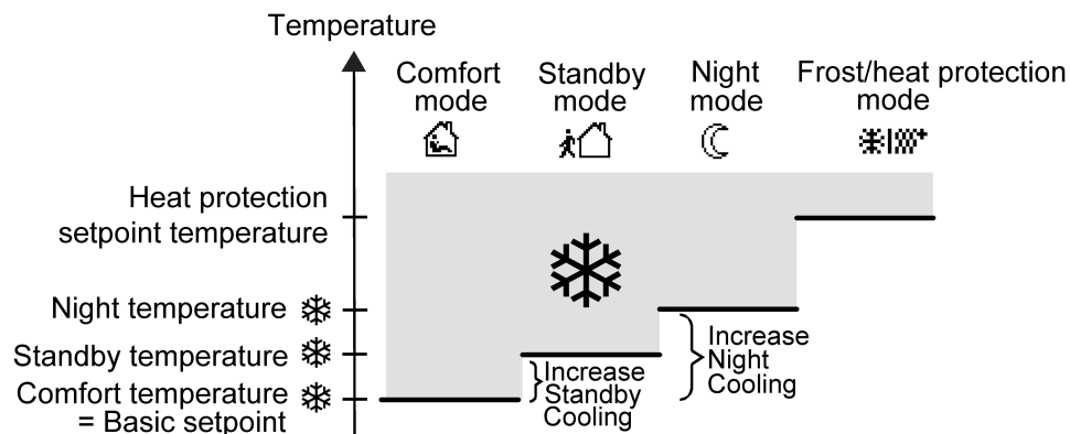
Figure 59: Setpoint temperatures in the operating mode "Cooling"
