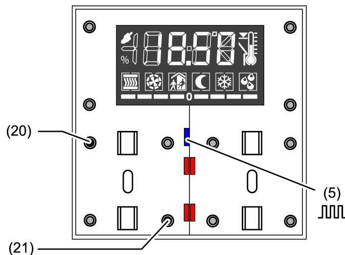
Figure 5: Activating programming mode
