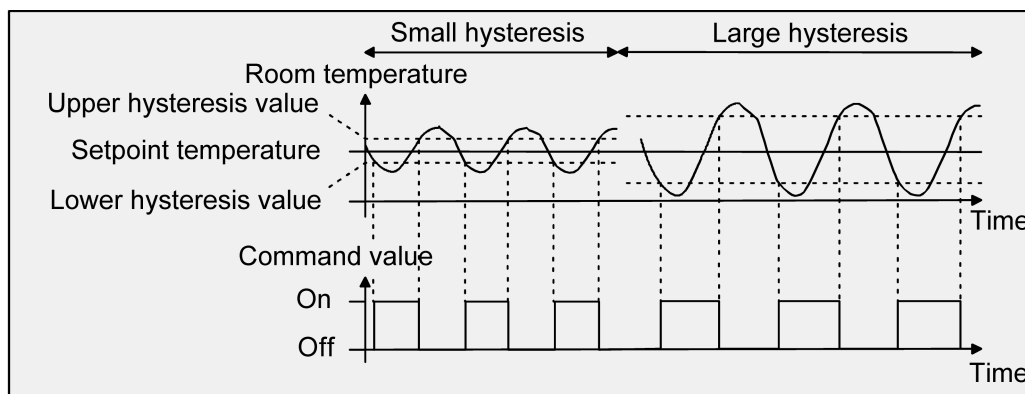
Figure 54: Effects of the hysteresis on the switching behaviour of a 2-point feedback control command value
