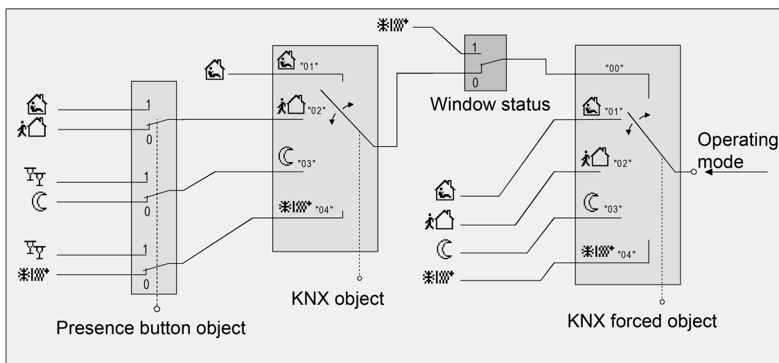
Figure 55: Operating mode switchover through KNX object with presence button
