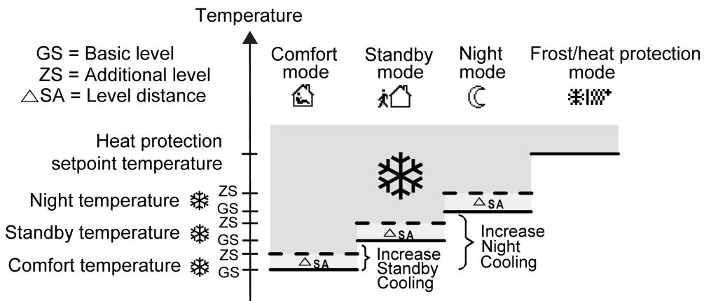
Figure 60: Setpoint temperatures in the operating mode "Basic and additional cooling"
