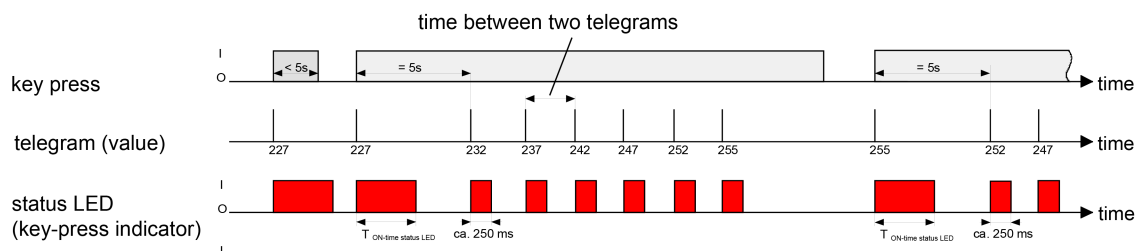
Figure 43: Example of value adjustment without value range overflow
