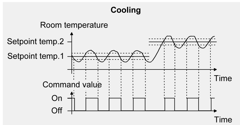
Figure 51: 2-point feedback control for the single "Cooling" operating mode
