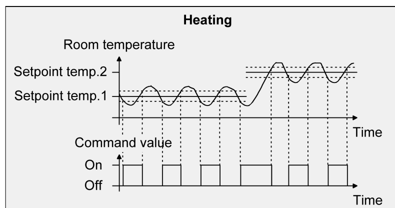
Figure 50: 2-point feedback control for the single "Heating" operating mode
