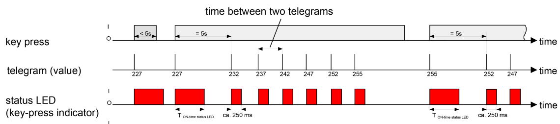
Figure 39: Example of value adjustment without value range overflow
