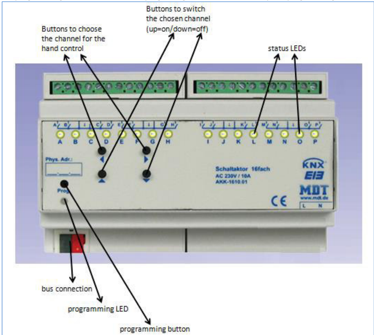
Figure 7: Overview hardware module switch actuator (e.g. AKK-1610.01)
