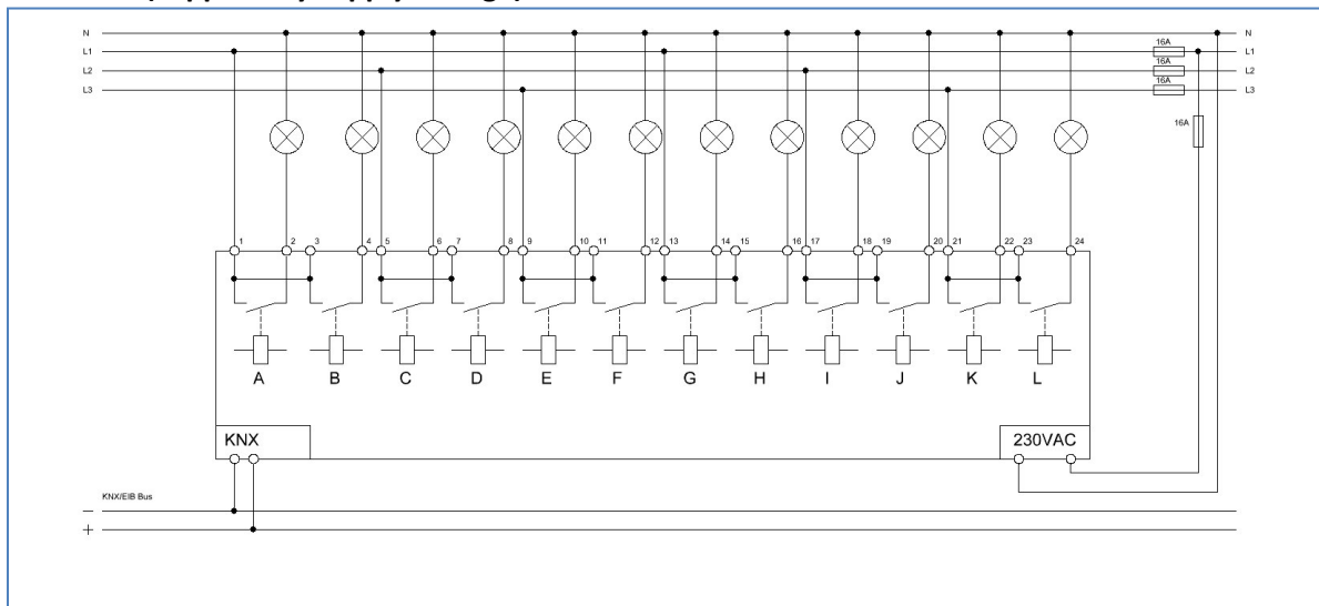
Figure 3: Exemplary circuit diagram AKS-1216.01
