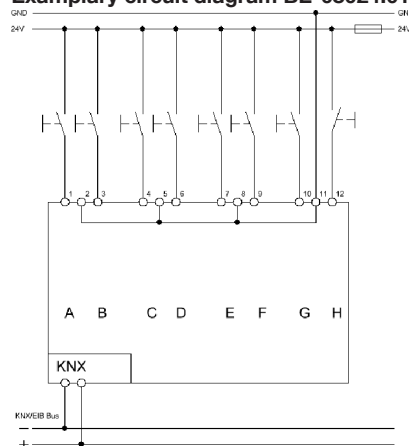
Exemplary circuit diagram BE-08024.01
