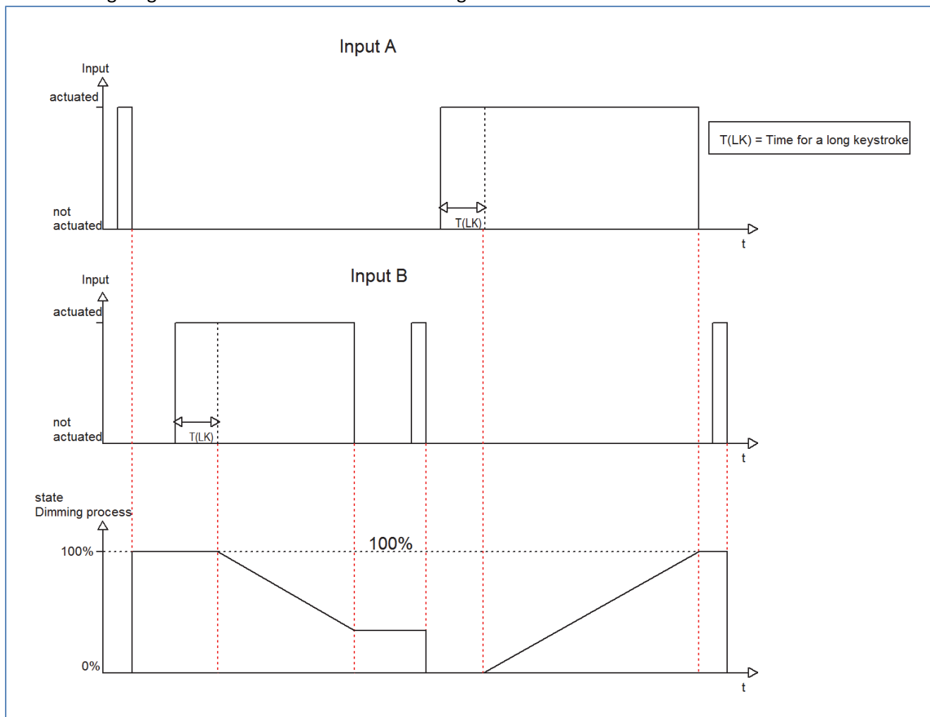
Chart 18: Dimming function
