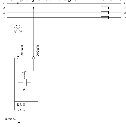
Exemplary circuit diagram AKK-01UP.01
