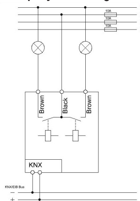
Exemplary circuit diagram AKK-02UP.01
