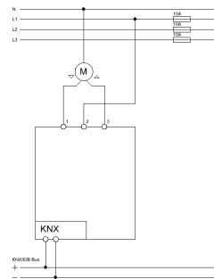
Anschluß JAL-01UP.01 - Exemplary circuit diagram JAL-01UP.01
