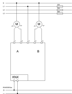
Anschluß JAL-0206.01 - Exemplary circuit diagram JAL-0206.01
