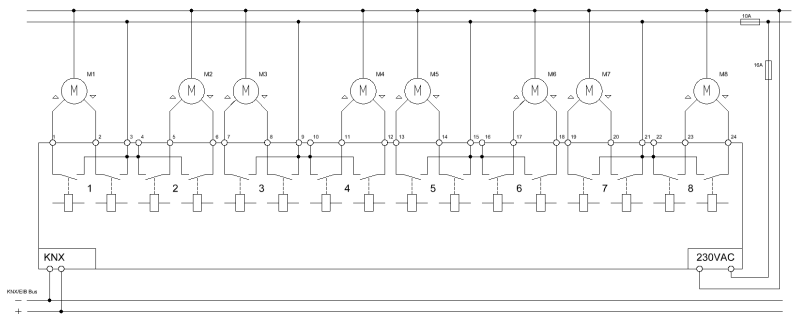
Anschluß JAL-0810.01 - Exemplary circuit diagram JAL-0810.01
