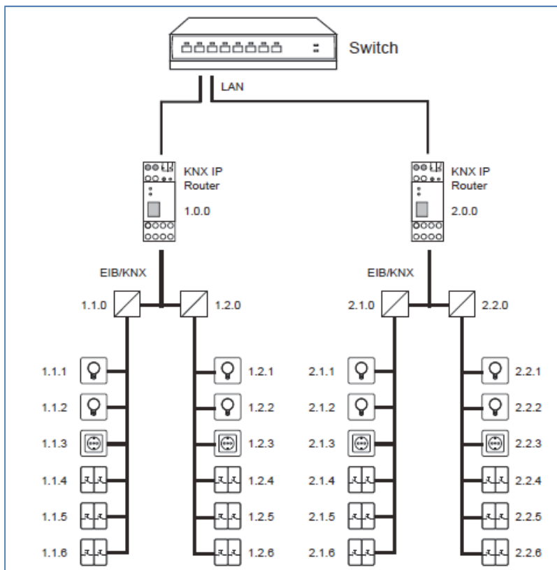
Figure 3: KNX IP Router as a backbone coupler
