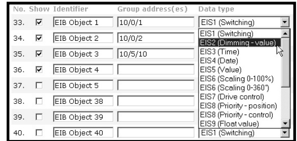
Setting up the EID data type
