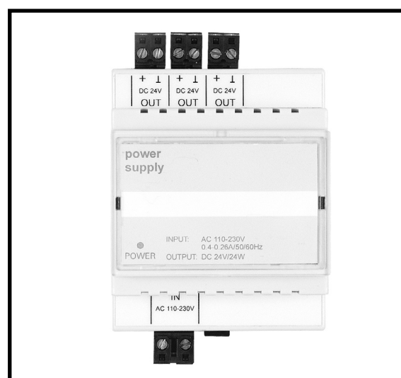
Power supply DC 24V REG-K
