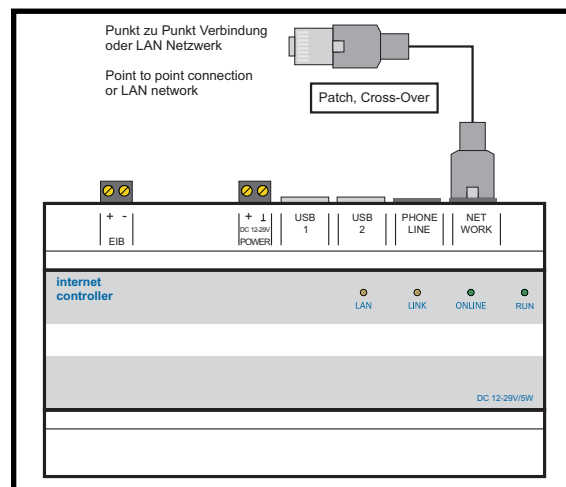
Connecting diagram LAN connection
