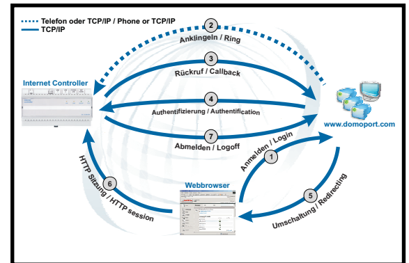
Communication between user, Domoport and IC 1 EIB
