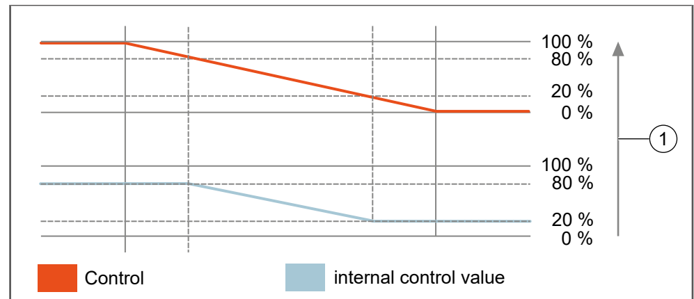
Fig. 42: Setting the maximum and minimum control value
