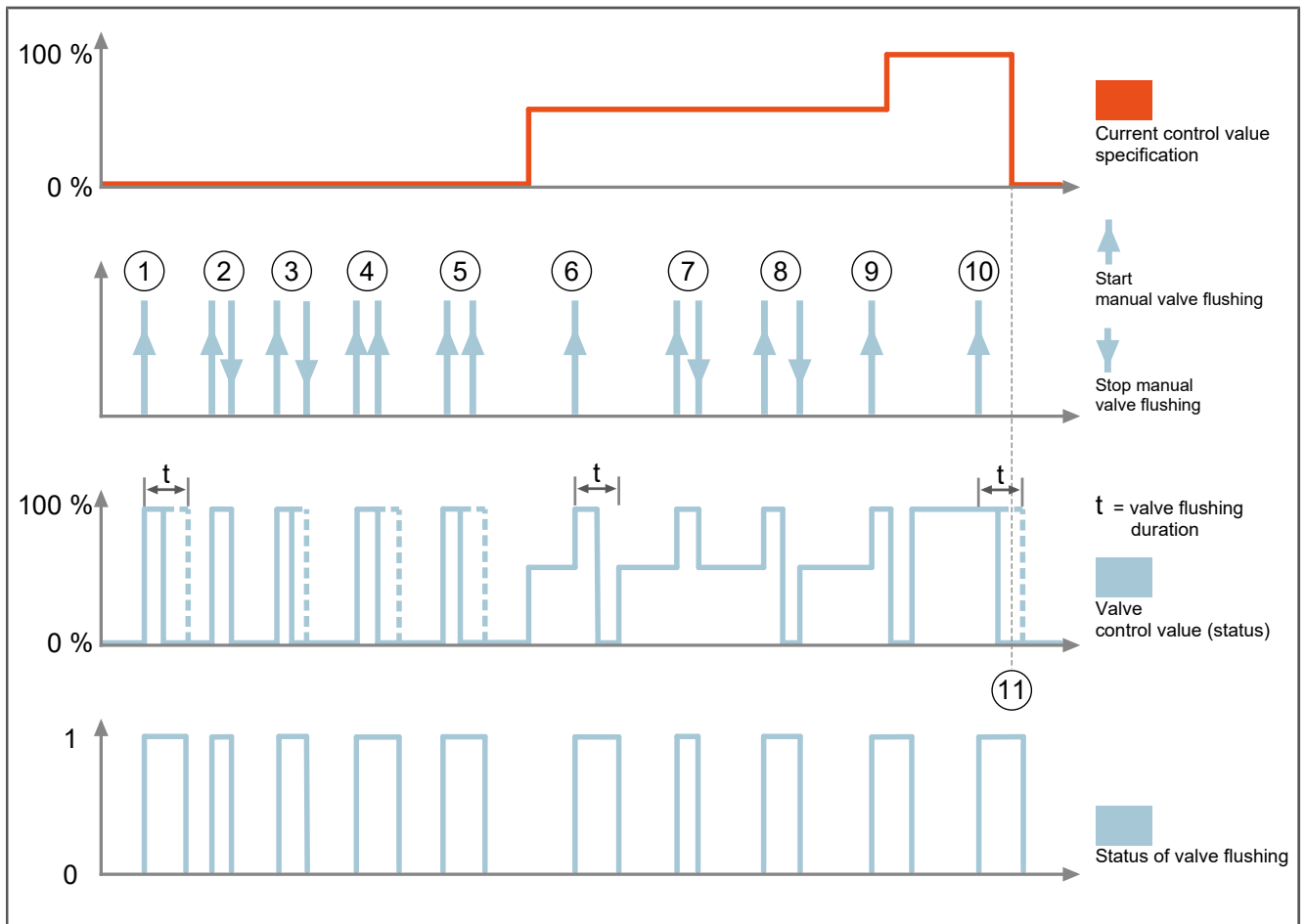
Fig. 21: Manual valve flushing process, illustration (examples):
