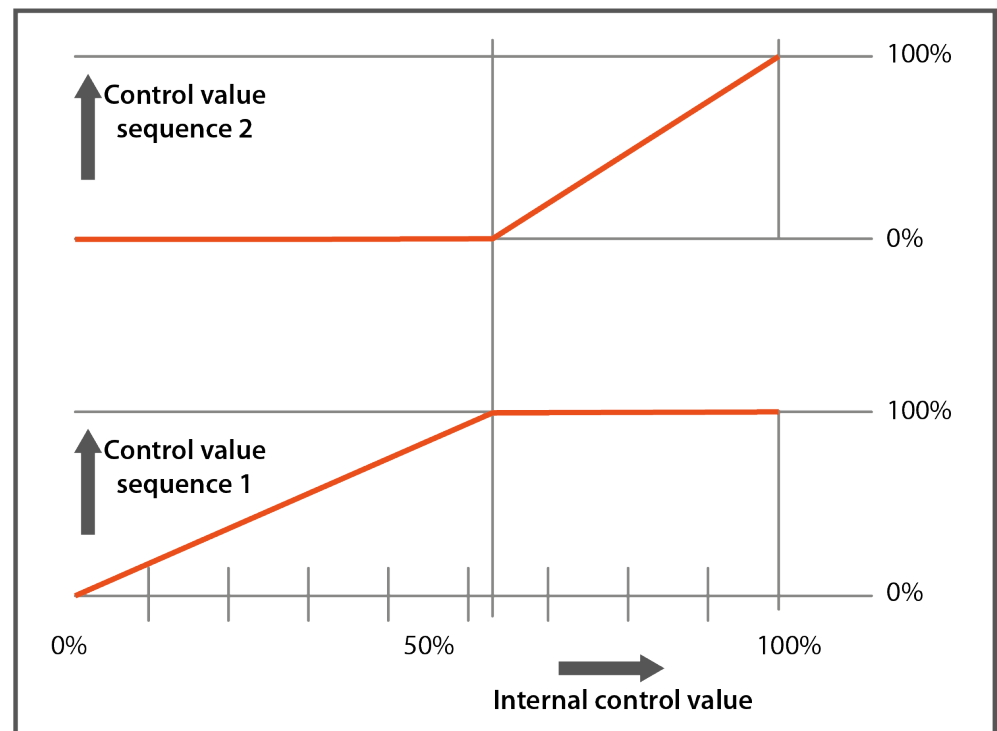
Fig. 27: Control values for sequence control
