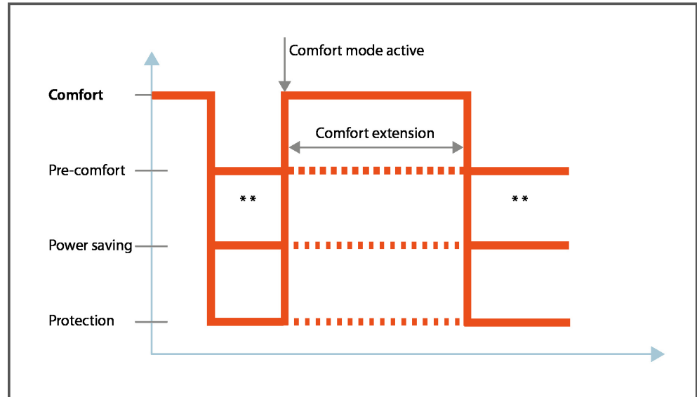
Fig. 32: Behavior if comfort mode is not set.
