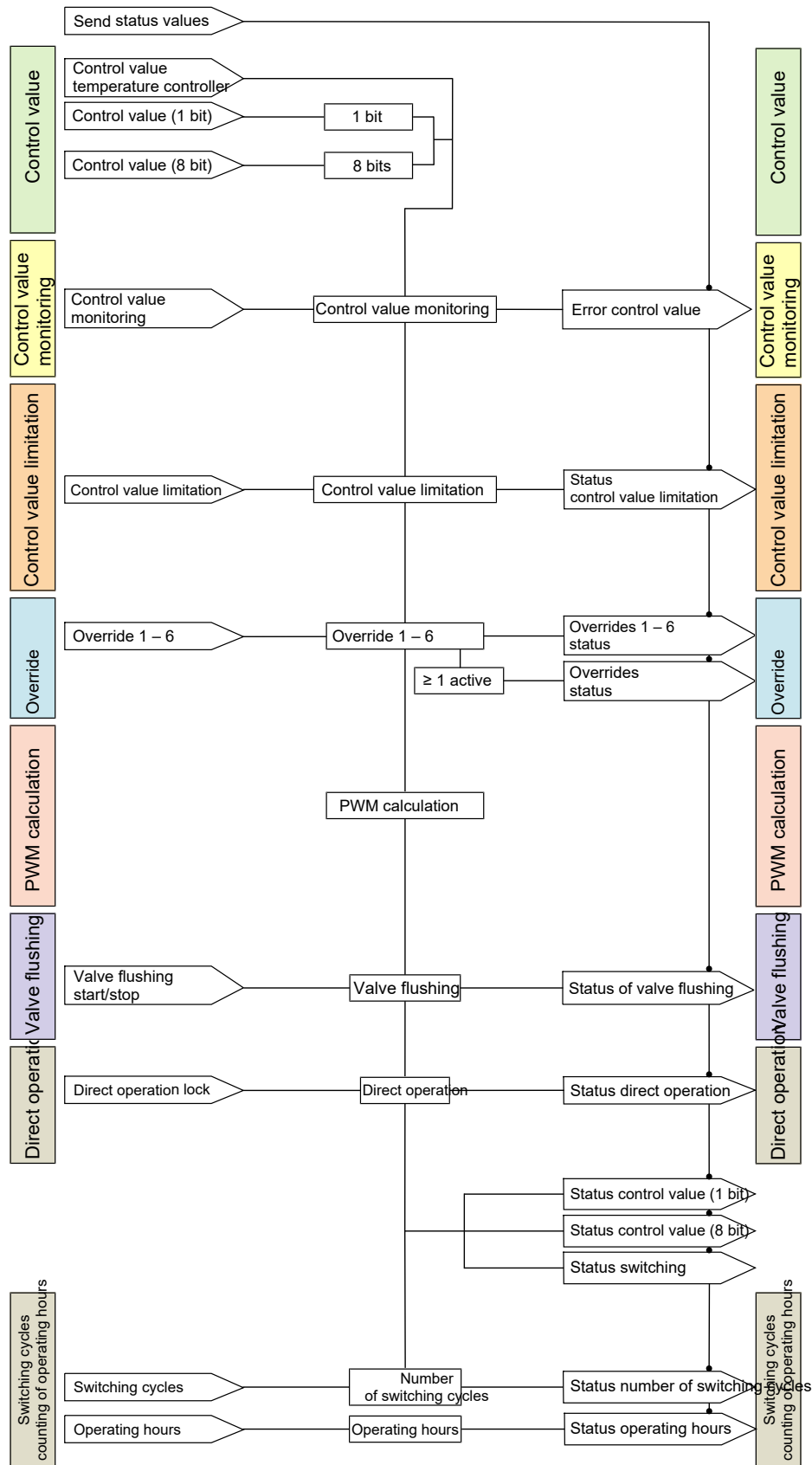
Fig. 12: Valve control flow chart
