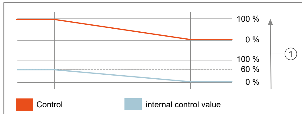
Fig. 40: Example 1: Scaling of the control value: 60 %
