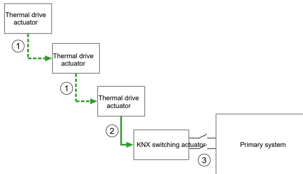
Fig. 43: Function overview of energy requirement request (cascading of thermal drive actuators)
