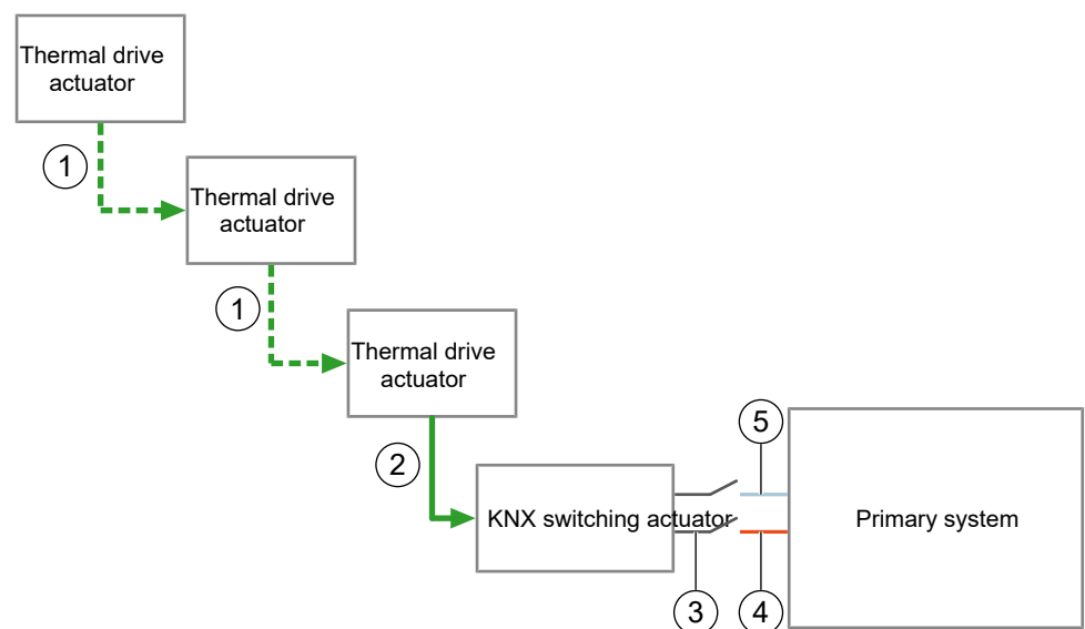
Fig. 44: Function overview of the pump control (cascading of thermal drive actuators)
