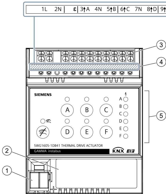
Fig. 3: Position and function of the connections and labeling, Thermal Drive Actuator N 605D41, 6 x AC 24...230 V
