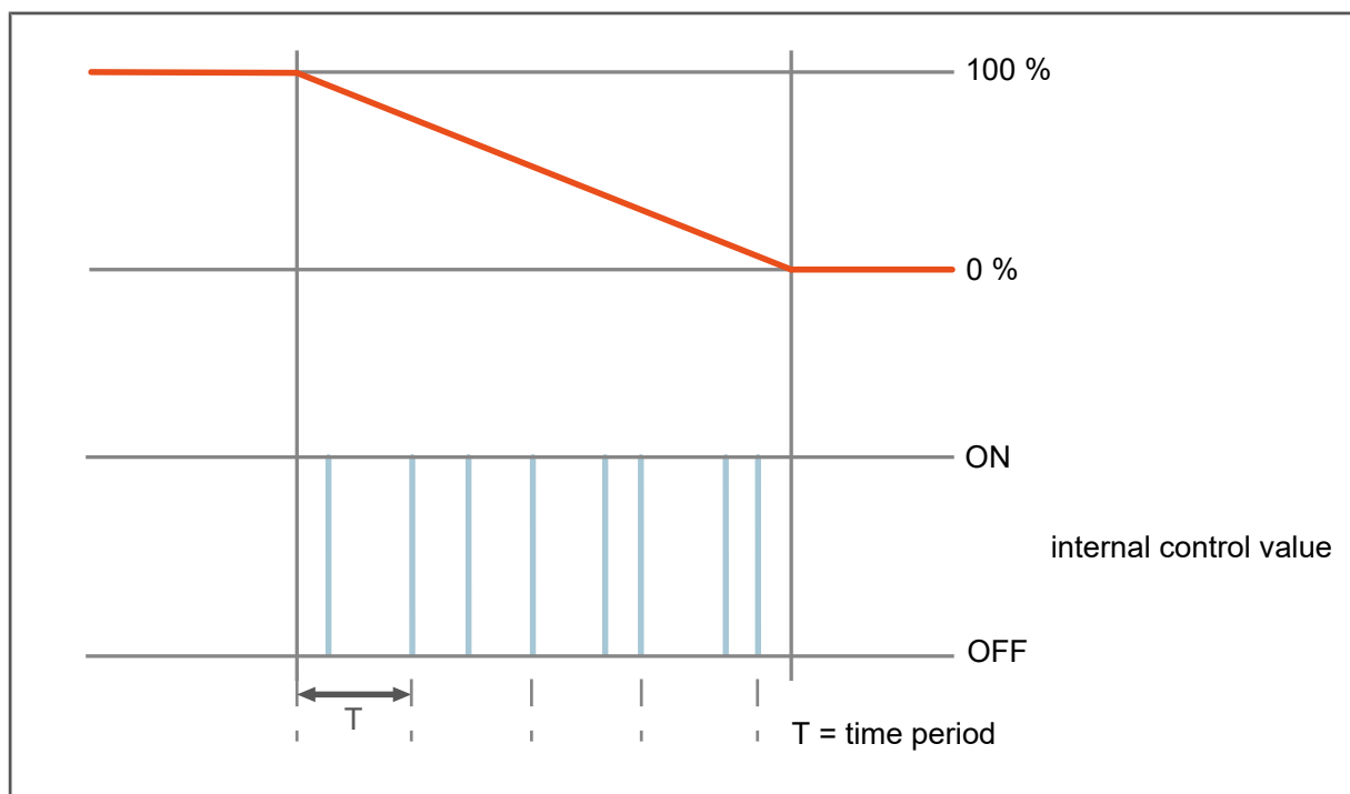
Fig. 39: Switching output of the control value
