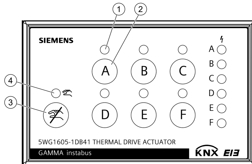
Fig. 22: Operation in direct operation, Thermal Drive Actuator N 605D41, 6 x AC 24...230 V
