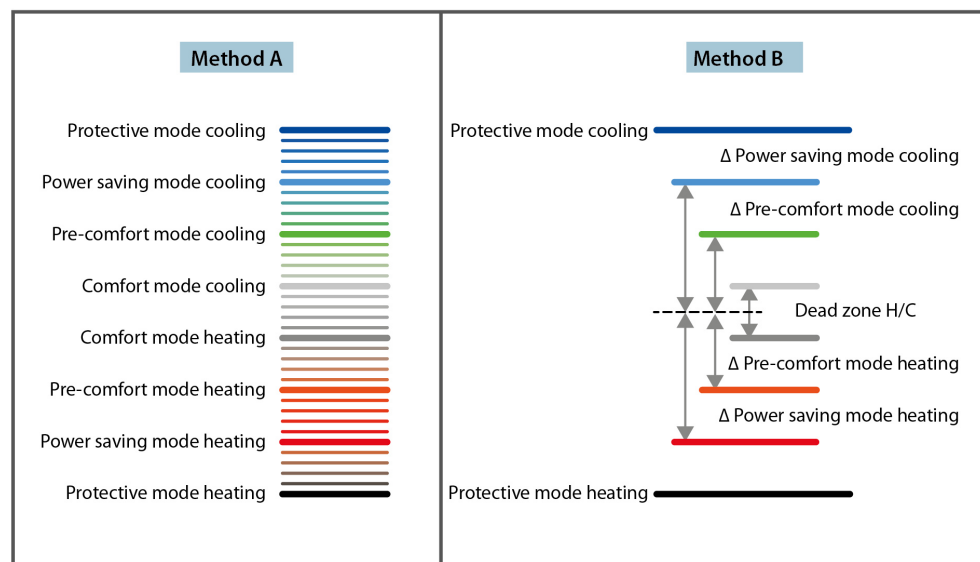
Fig. 28: Methods for setting a setpoint
