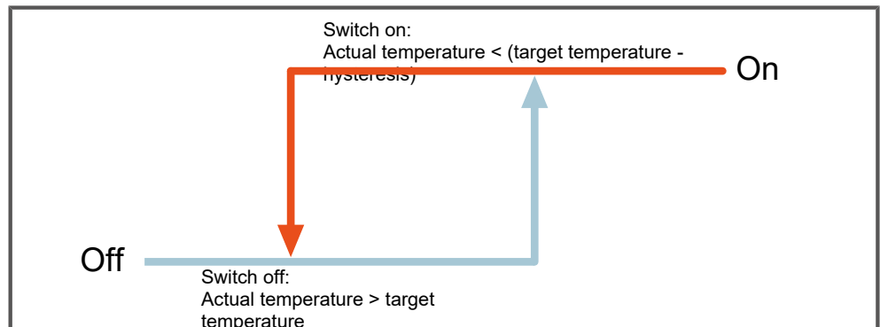
Fig. 23: 2-point control for "Heating"
