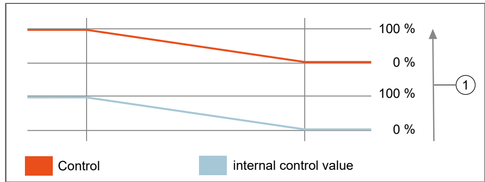
Fig. 37: Valve completely open above 100 %, closed below 1 %
