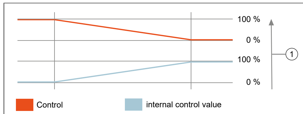
Fig. 41: Example 2: Scaling of the control value: 100 %, inverted control value
