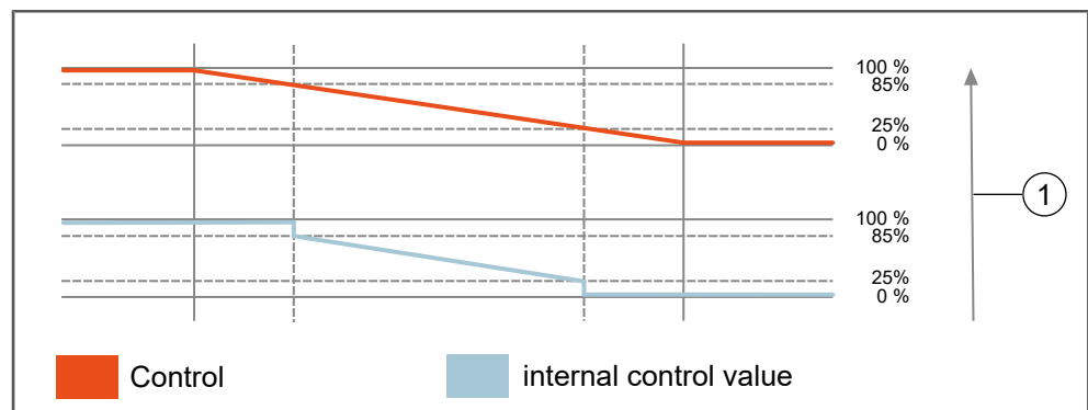
Fig. 38: Valve completely open above 85 %, closed below 25 %
