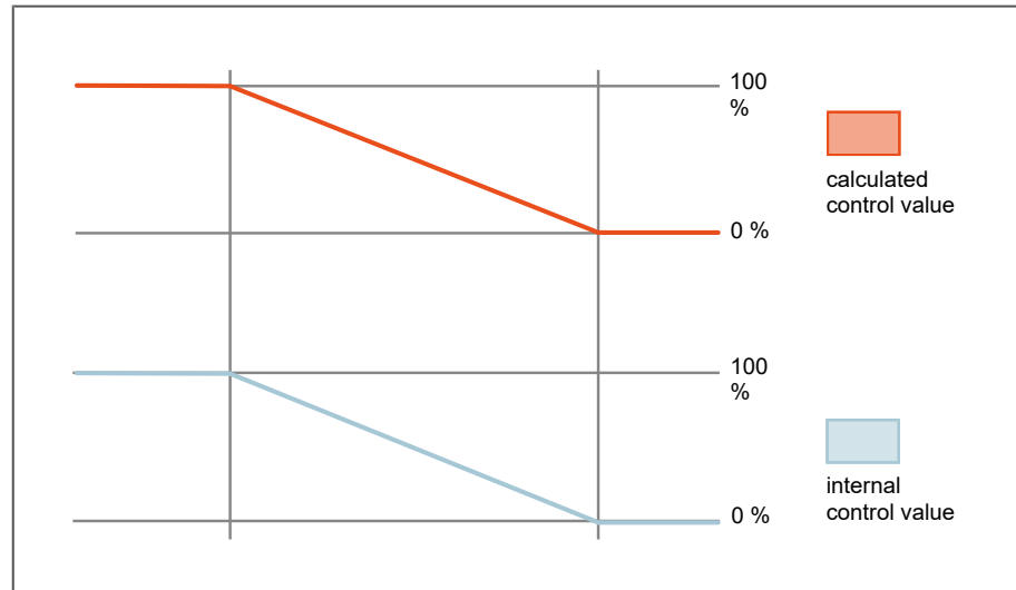
Fig. 25: PI control with continuous control value
