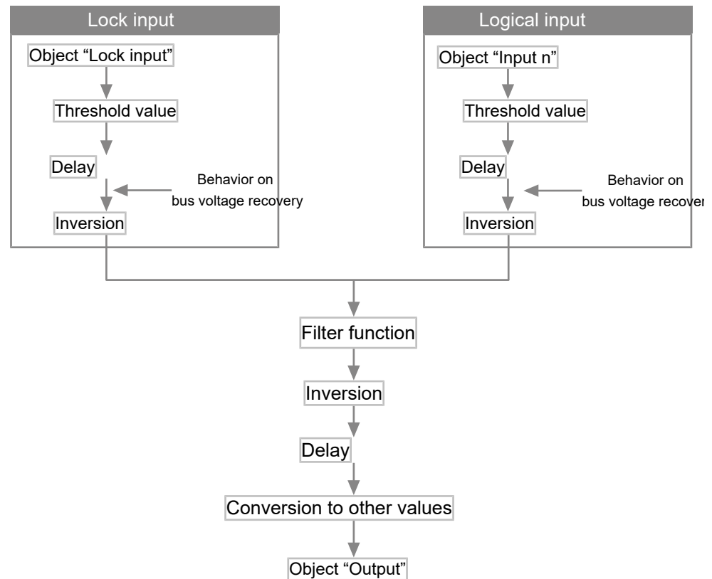
Fig. 52: Process diagram for LOCK
