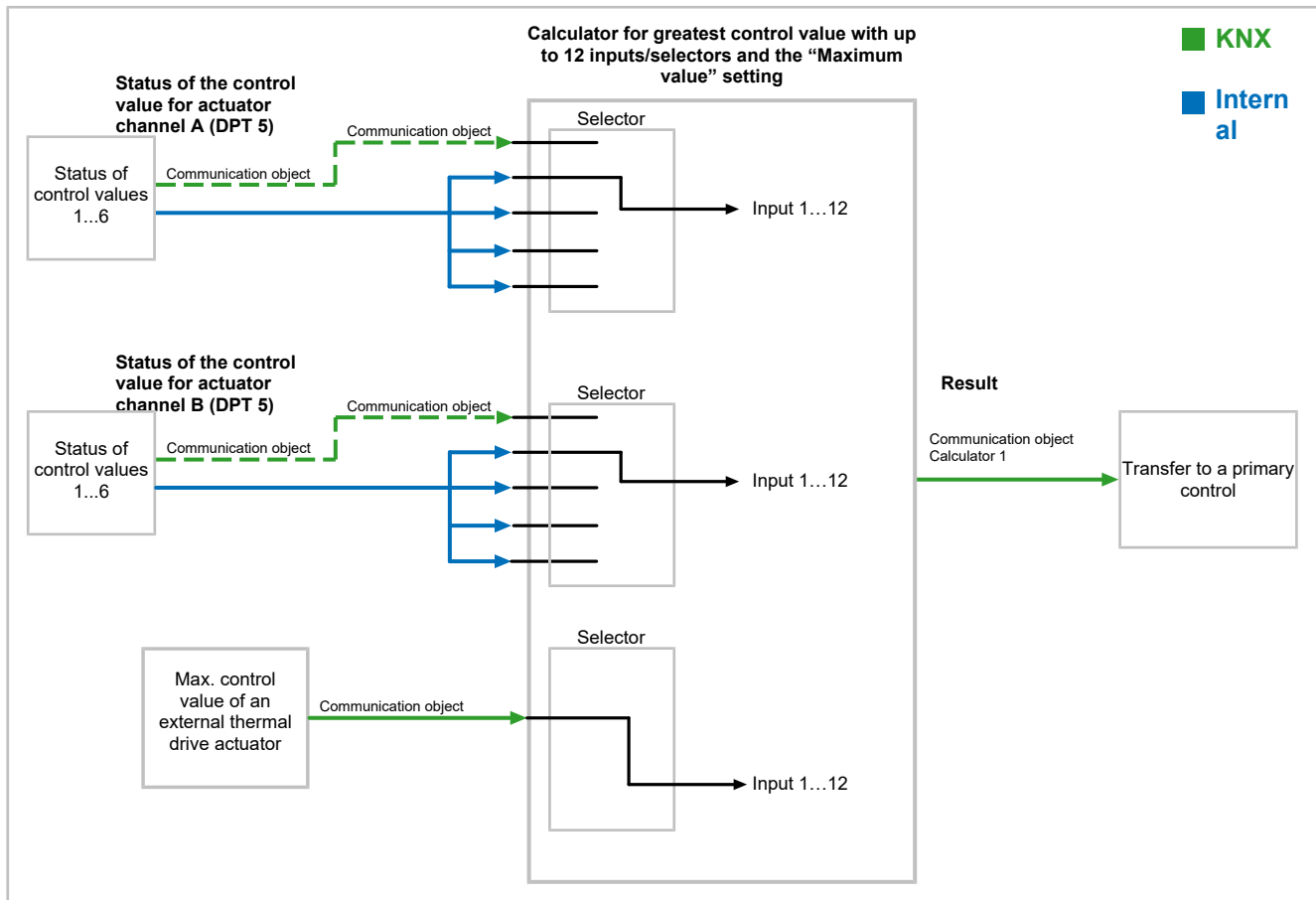
Fig. 45: Evaluation of the greatest control value (example)
