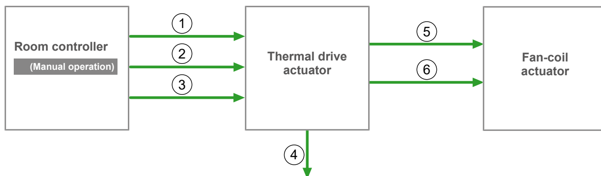
Fig. 36: Automatic activation of the fan levels
