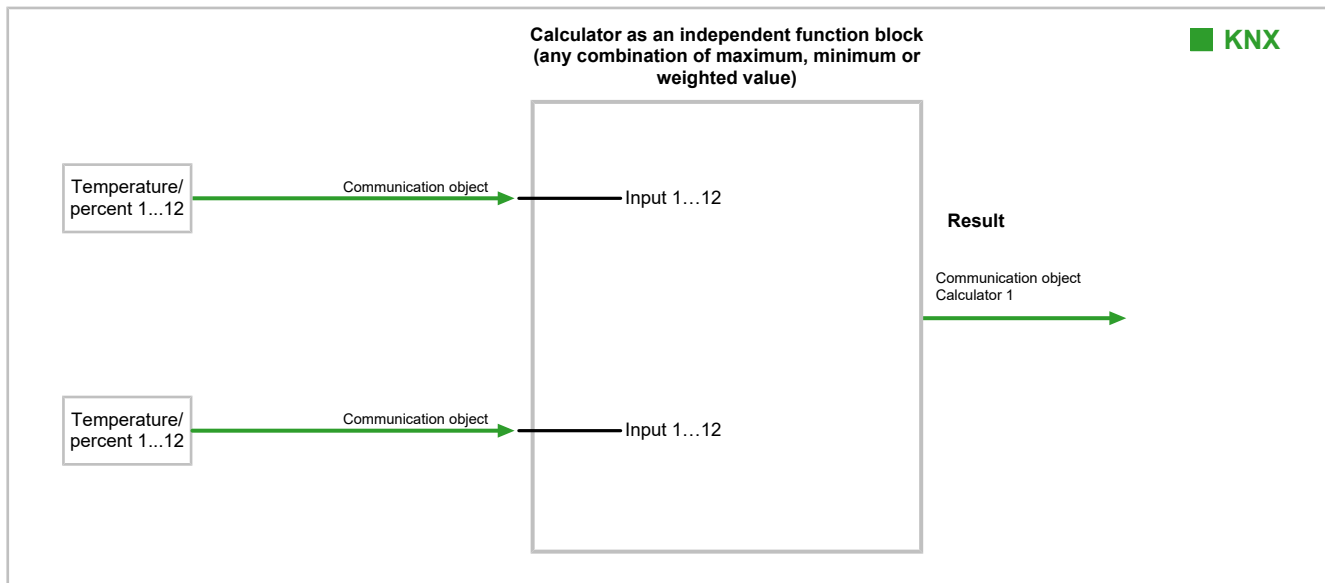
Fig. 47: Using the calculator as a stand-alone unit (example)
