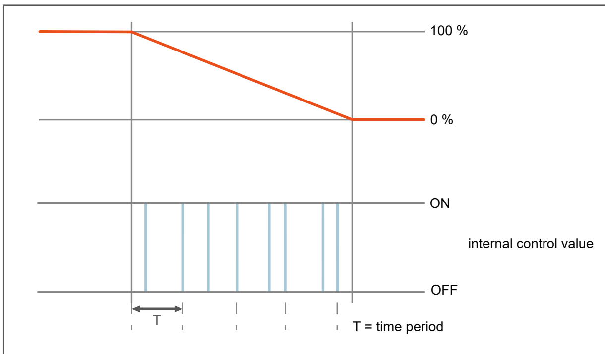
Fig. 26: PI control with On/Off command
