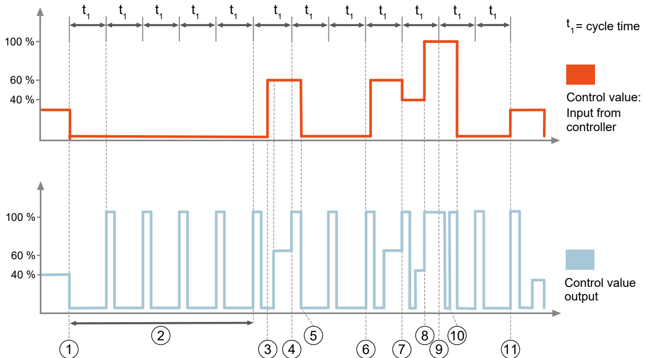
Fig. 19: Cyclic valve flushing process (triggered automatically), graphic display (example)
