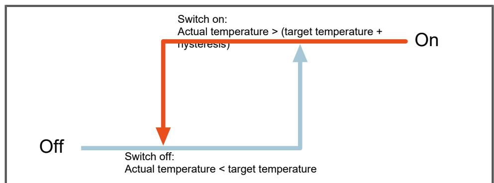
Fig. 24: 2-point control for "Cooling"
