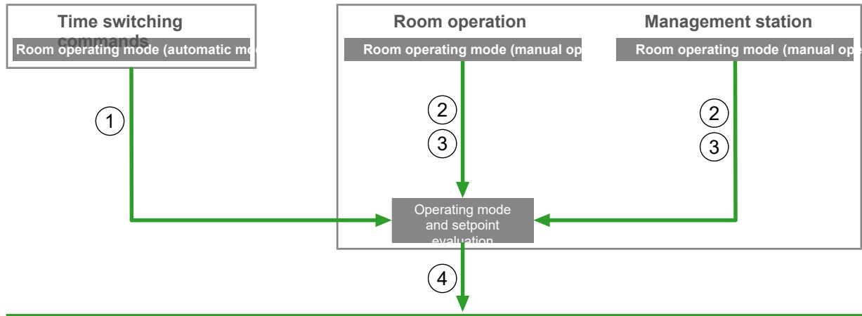
Fig. 30: Switching room operating modes
