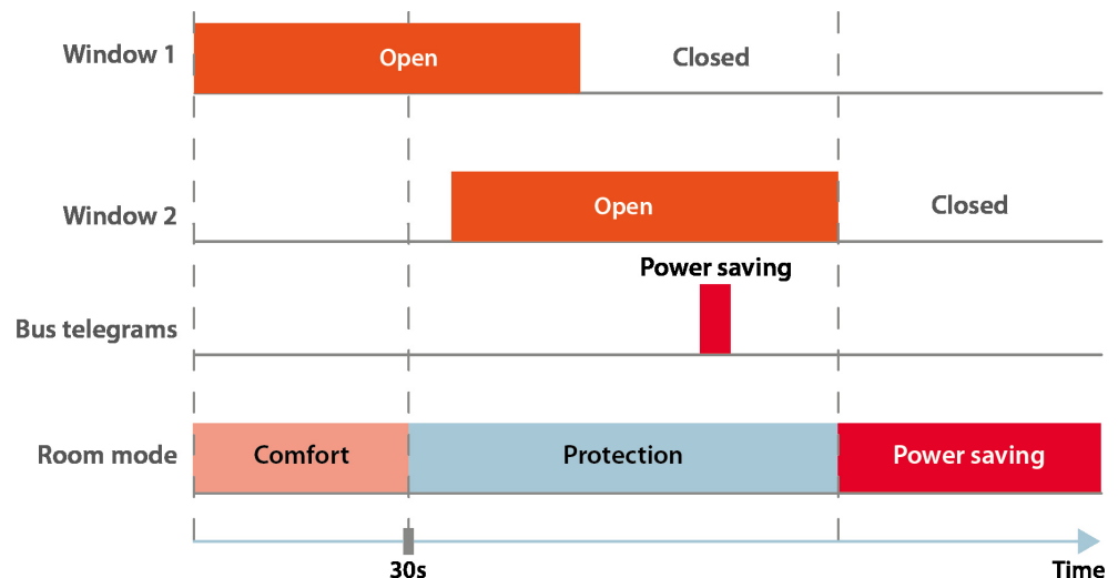
Fig. 35: Evaluation of the window statuses (example with 30 s)
