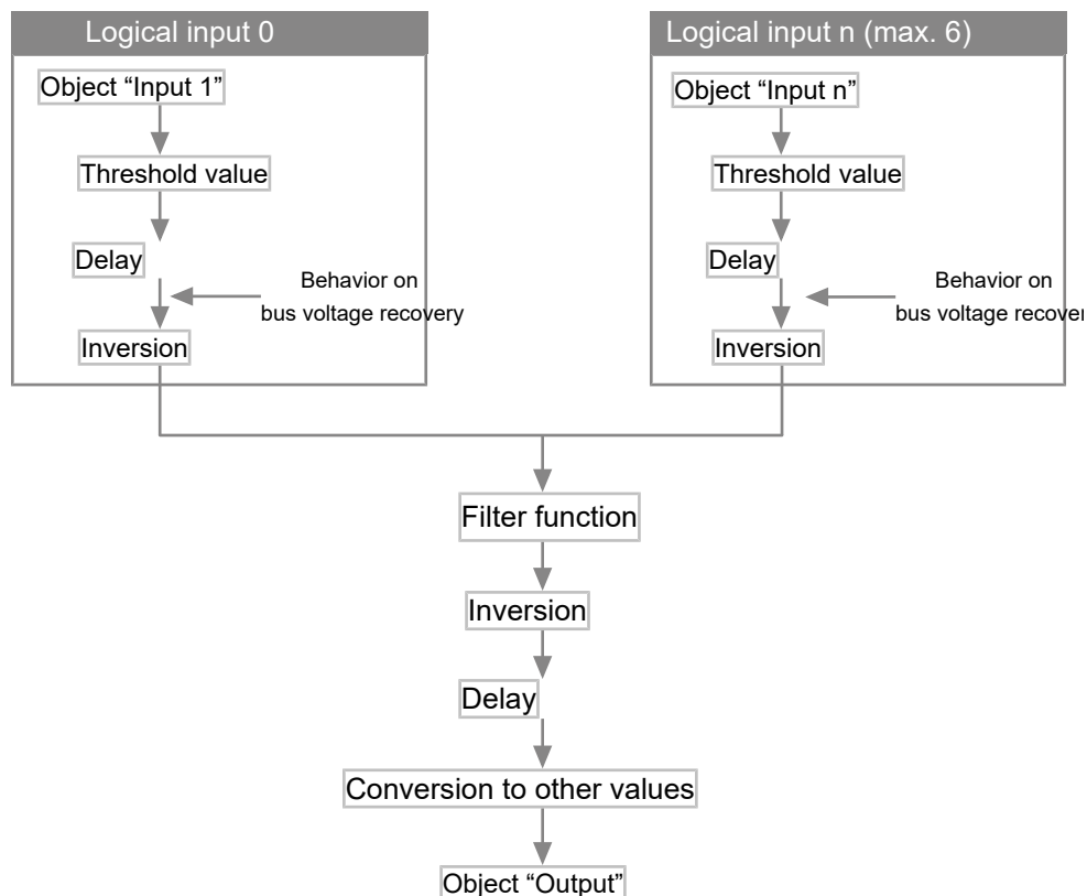
Fig. 49: Process diagram for [AND, OR, XOR, TRIGGER]
