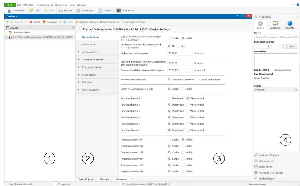
Fig. 5: User interface
