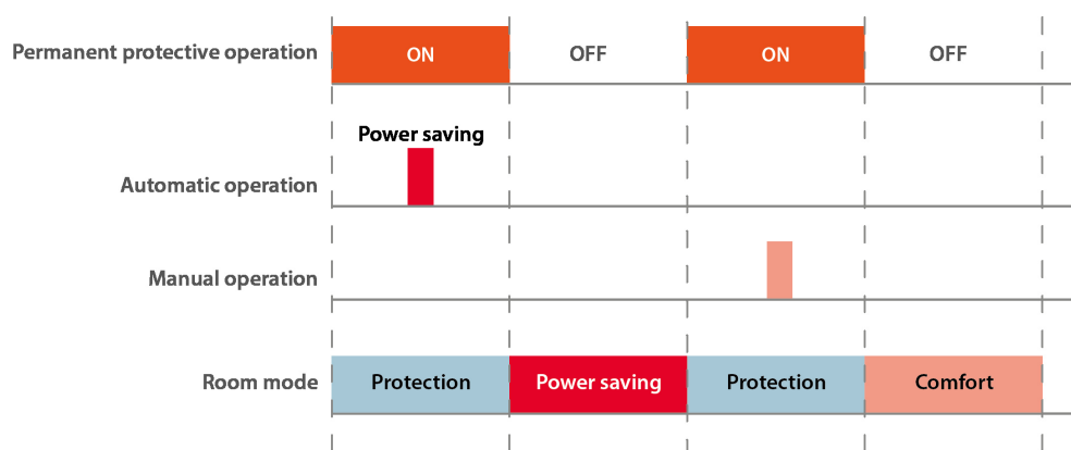
Fig. 33: Activating and deactivating permanent protection mode
