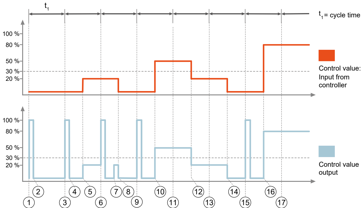
Fig. 20: Intelligent valve flushing process, illustration (example):
