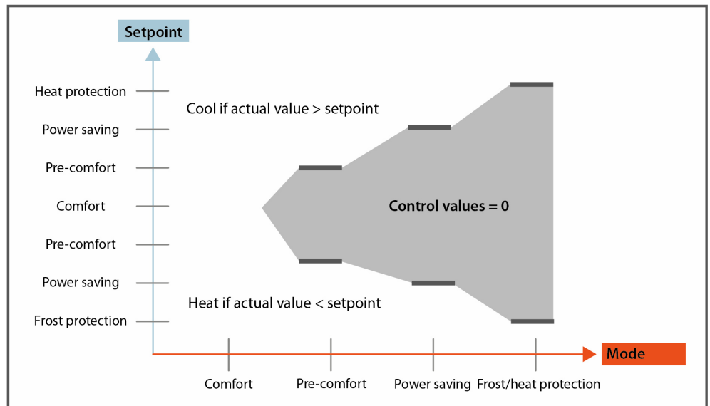
Fig. 29: Setpoint setting via basic setpoint + setpoint shift
