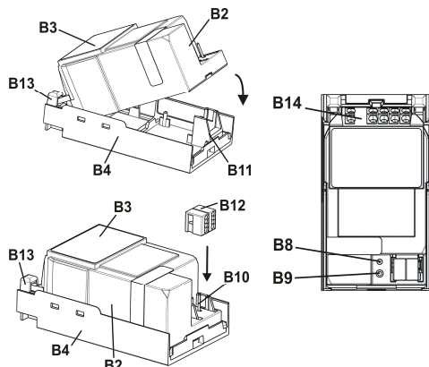
figure 7: mounting of an RL module
