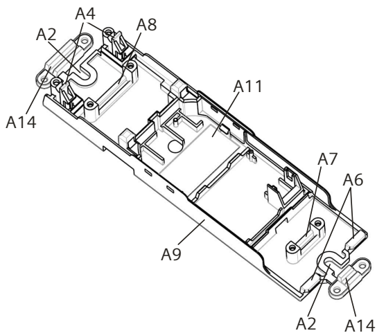
figure 2b: Mounting
