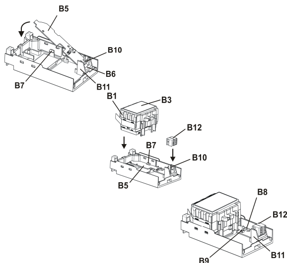
figure 5: mounting of a RS module
