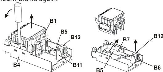
figure 6: dismounting an RS module
