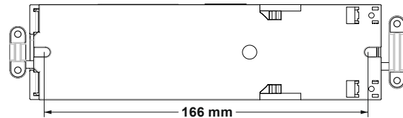
figure 2a: Mounting
