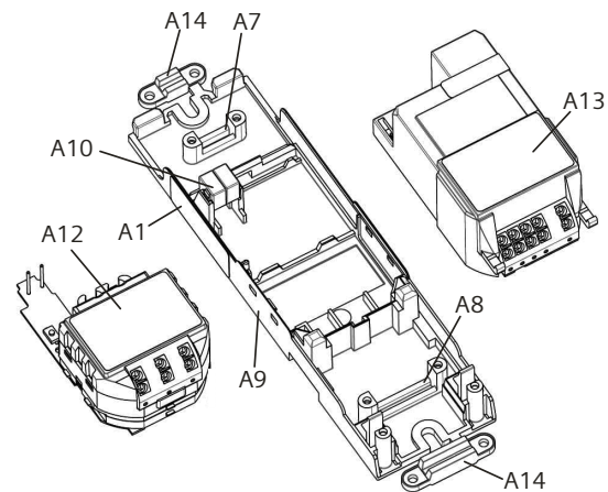
figure 4: mounting / dismounting of RS/RL modules
