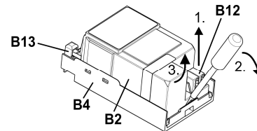
figure 8: dismounting an RL module
