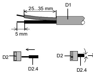
figure 10: Connecting / Disconnecting bus cables
