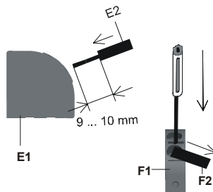
figure 11: Connecting/disconnecting mains and load circuit
