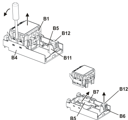
figure 7: Dismounting of a RS module
