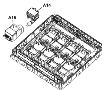
figure 5: Mounting / Dismounting of RS / RL modules
