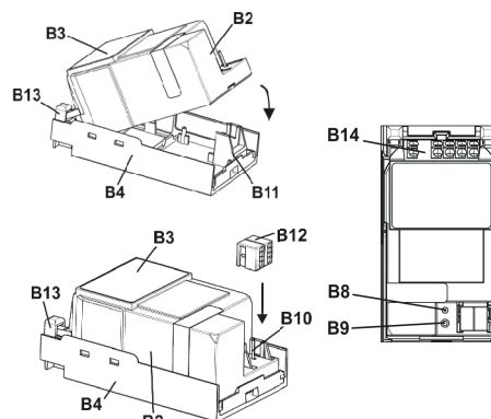
figure 8: Mounting of an RL module
