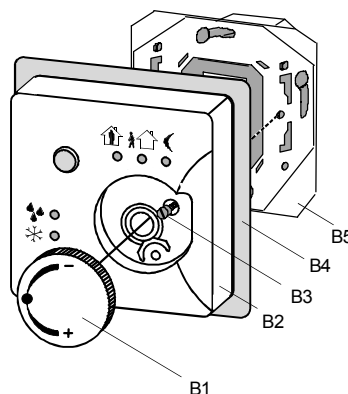
Diagram 3: Installing the temperature controller
