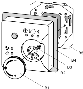
Diagram 1: Installation of the temperature controller
