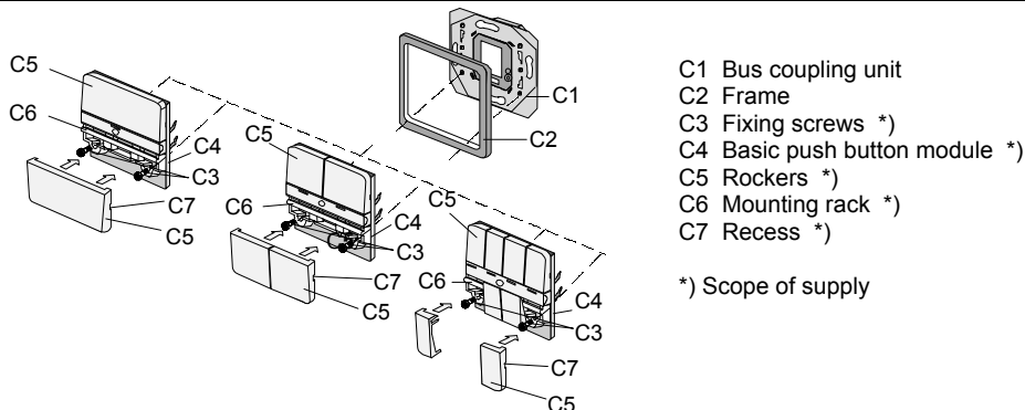
Diagram 1: Push button UP with infrared receiver
