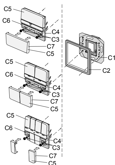
Diagram 3: mounting sequence
