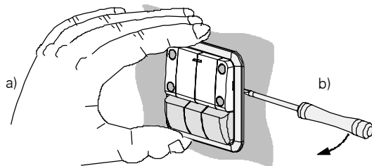
Diagram 7: Dismantling
