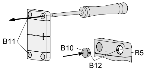
Diagram 6: Inserting / changing pictograms
