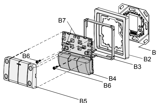
Diagram 4: Mounting sequence
