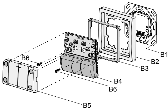
Diagram 1: Mounting the push button UP 230
