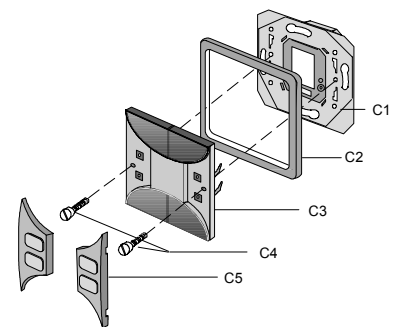
Figure 2: Mounting the push button (basic representation)
