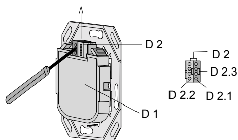
Diagram 7: Removing the bus terminal
