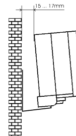
Figure 2: Adapting the mounting bracket
