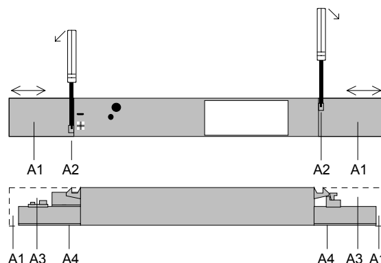
Figure 2: Opening and closing the covers
