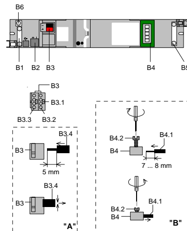
Diagram 3: Connections
