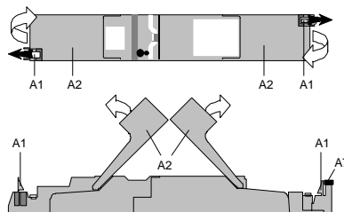
Diagram 2: Opening and closing the hinged covers
