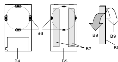
Figure 2: Mounting the IR transmitter
