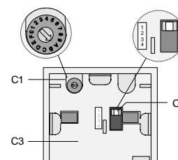
Figure 3: Adjusting the transmission channel
