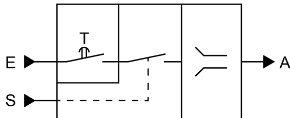
Image 22: Disabling element [Filtering/Time]
