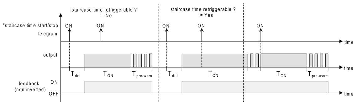
Image 1: Switch-on behaviour of the staircase function
