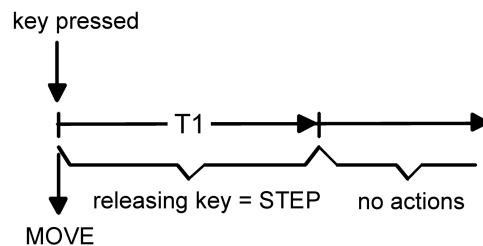
Image 10: Operation concept "long – short"
