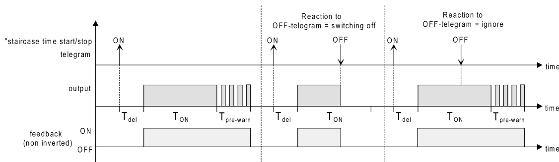
Image 2: Switch-off behaviour of the staircase function
