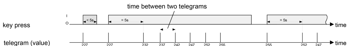
Image 13: Example of value adjustment without value range overflow
