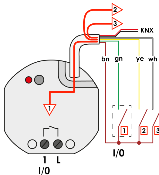
Image 7: Functionality of the input 1 when controlling the internal switching output as single-area operation
