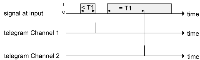
Image 19: Example of operation concept "Channel 1 or Channel 2"
