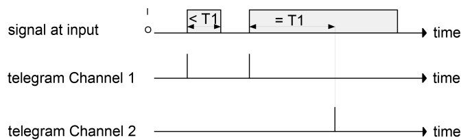
Image 20: Example for operation concept "Channel 1 and channel 2"
