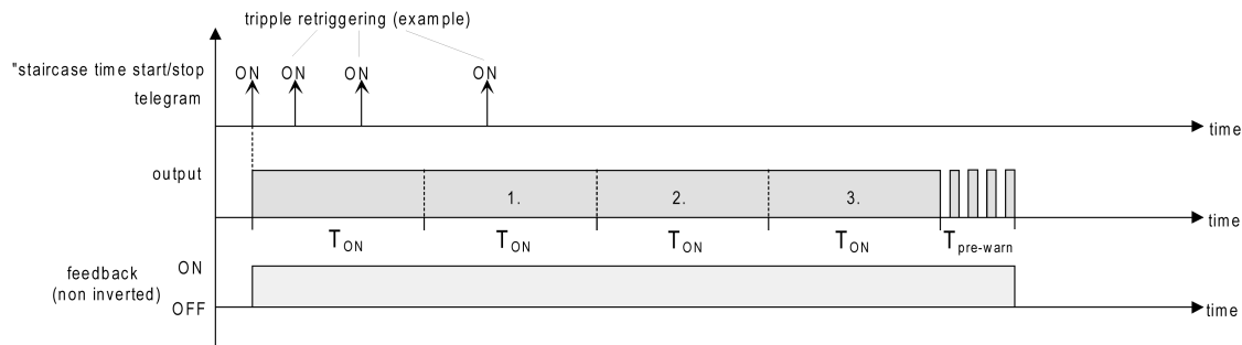
Image 4: Time extension of the staircase function
