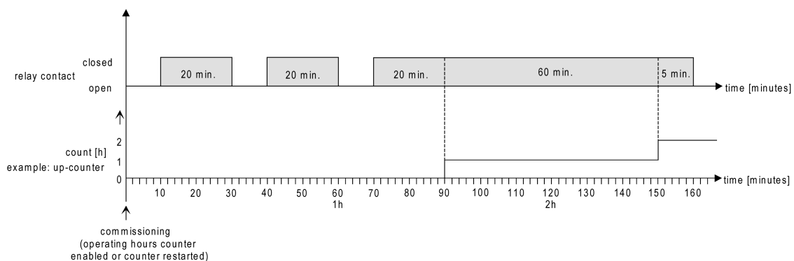
Image 6: Function of the operating hours counter (using the example of counted hours)
