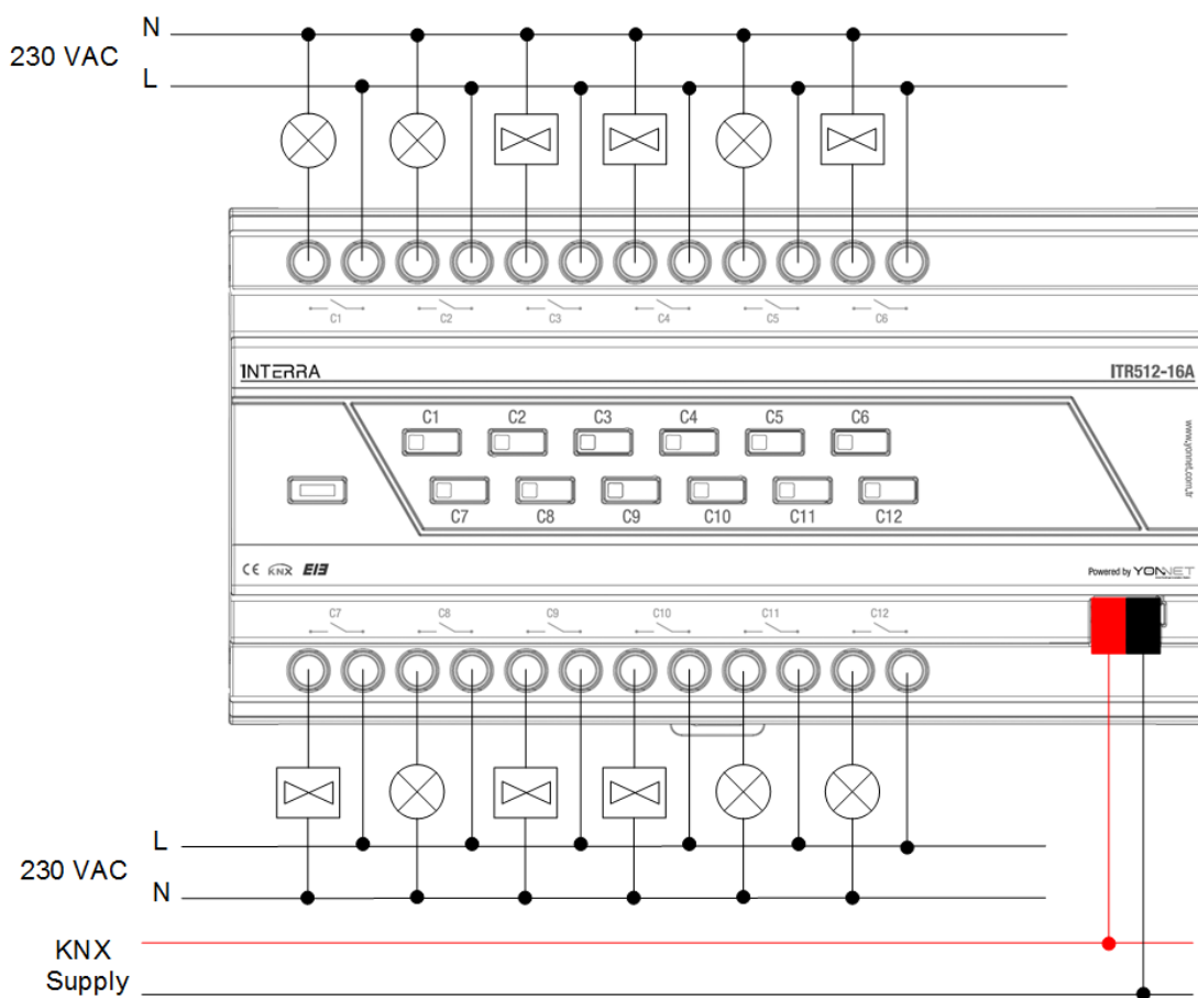
Fig21. Connection Diagram Example Configuration 1
