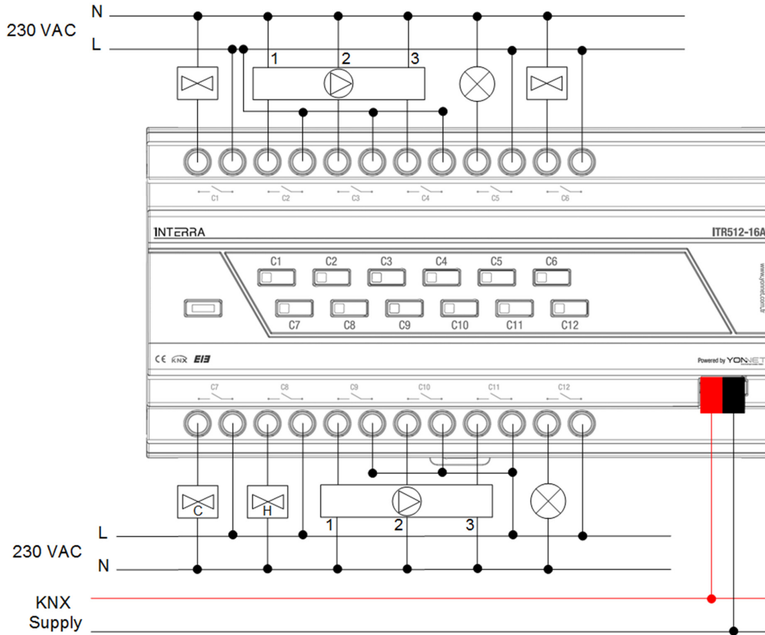
Fig22. Connection Diagram Example Configuration 2
