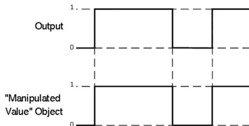
Fig11. Manipulated Value (1 Bit)
