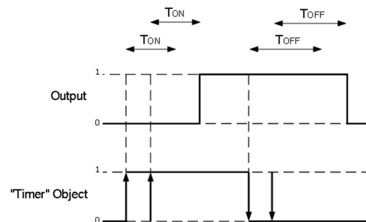
Fig5. ON/OFF Delays Retriggerable
