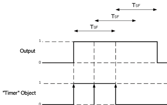
Fig3. Staircase Function Retriggerable
