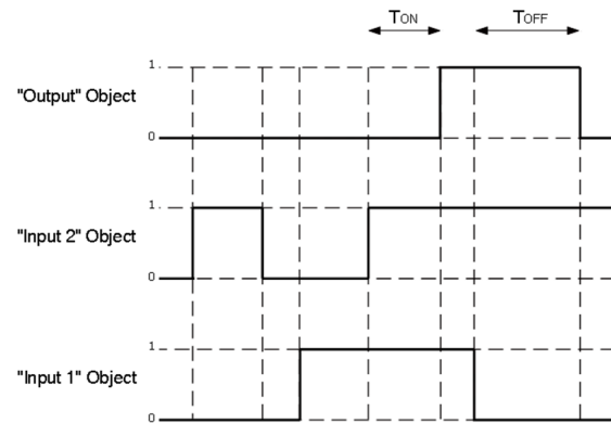
Fig1. Logic Gate with delays
