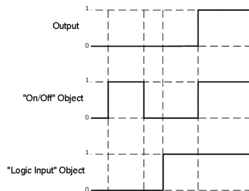
Fig8. AND Logic Function
