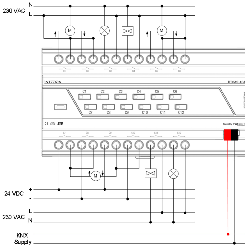
Fig23. Connection Diagram Example Configuration 3
