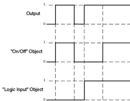
Fig9. OR Logic Function
