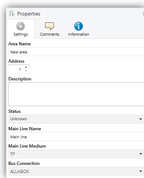
Figure 11. ETS parallel downloads configuration.
