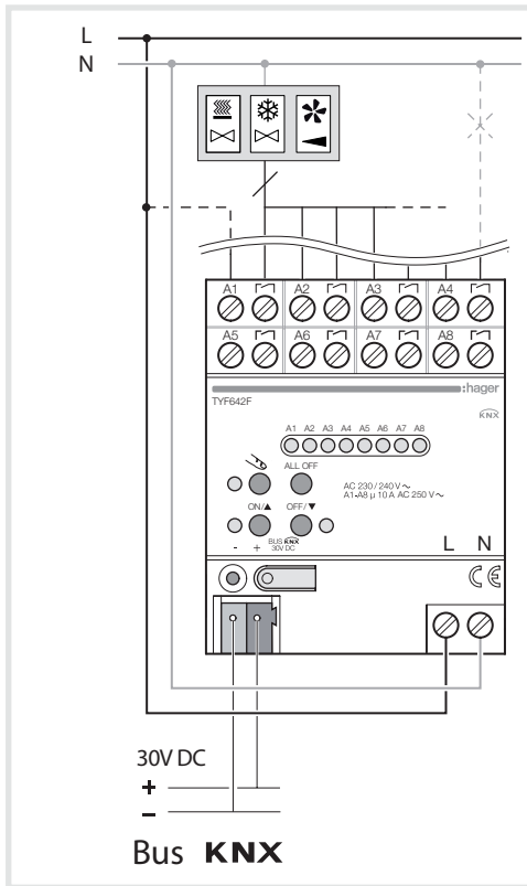
Connection diagram (Fig. 3)
