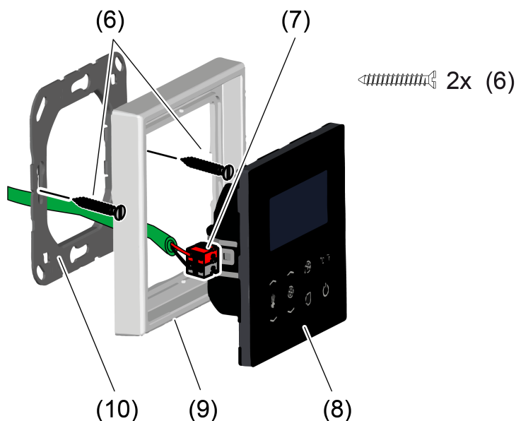
Image 4: Device fitting
