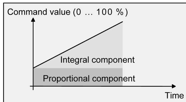
Image 41: Continuous PI control
