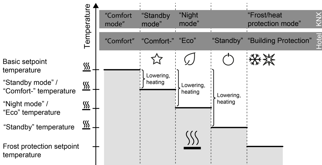
Image 47: Setpoint temperatures in the operating mode "Heating"
