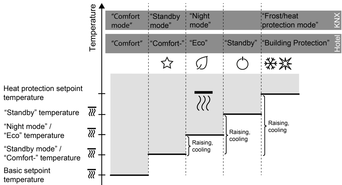
Image 48: Setpoint temperatures in the operating mode "Cooling"
