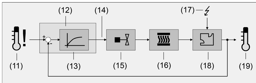
Image 40: Controlled system of single-room temperature control
