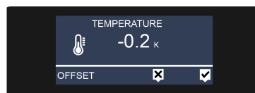
Image 31: Setting, temperature measurement offset (menu level 2)
