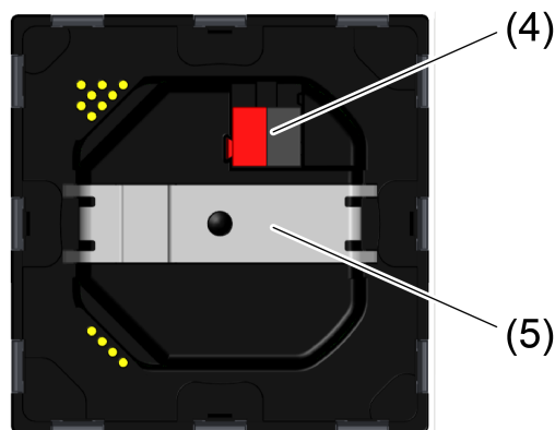
Image 2: Device view, rear side
