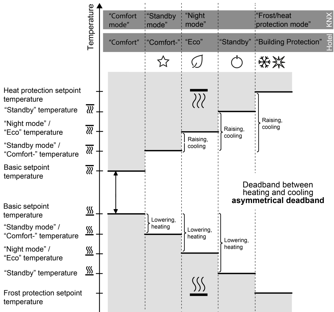
Image 49: Setpoint temperatures in the operating mode "Heating and cooling" with asymmetrical deadband
