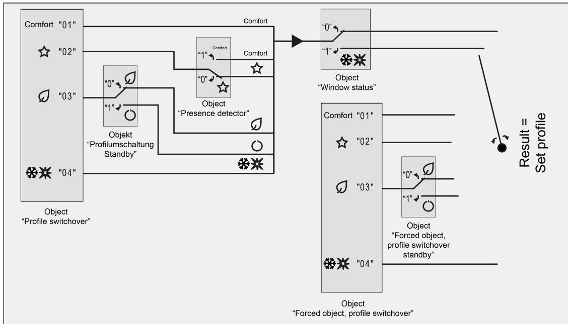
Image 45: Profile switchover through KNX objects with presence detector
