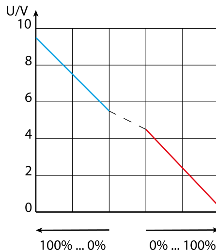
Image 50: Valve characteristic, example Belparts
