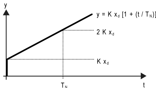
Image 43: Function of the command value of a PI control
