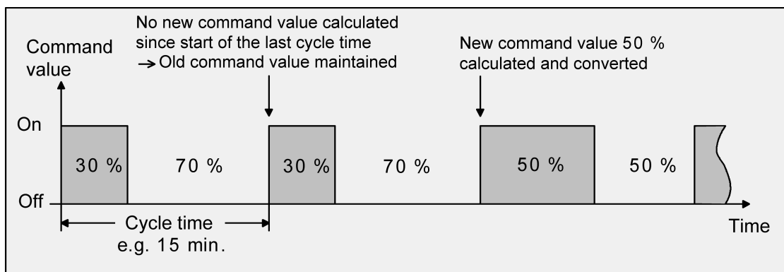
Image 42: Switching PI control
