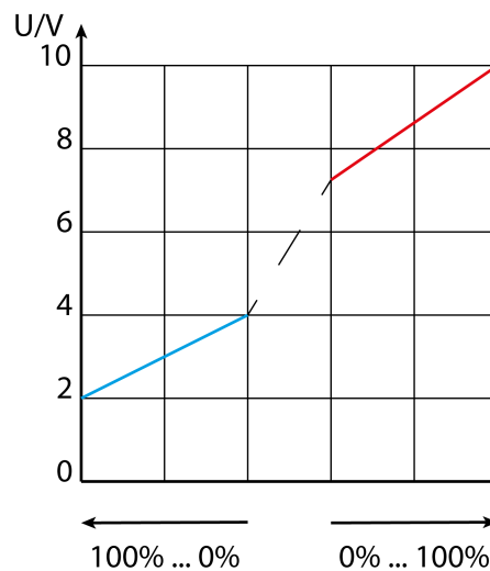
Image 51: Valve characteristic, example Swegon
